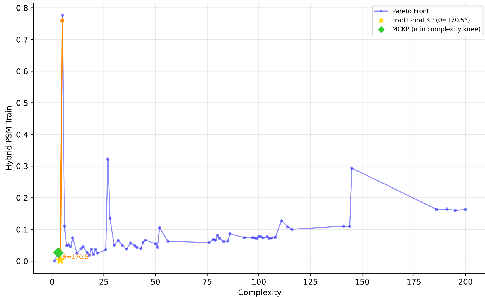
228_elusage - Run 30 - MVP - Hybrid PSM Train \lambda_1=0.00, \lambda_2=0.30, \lambda_3=0.00 | Difficulty: 0.45 | Method: mckp
