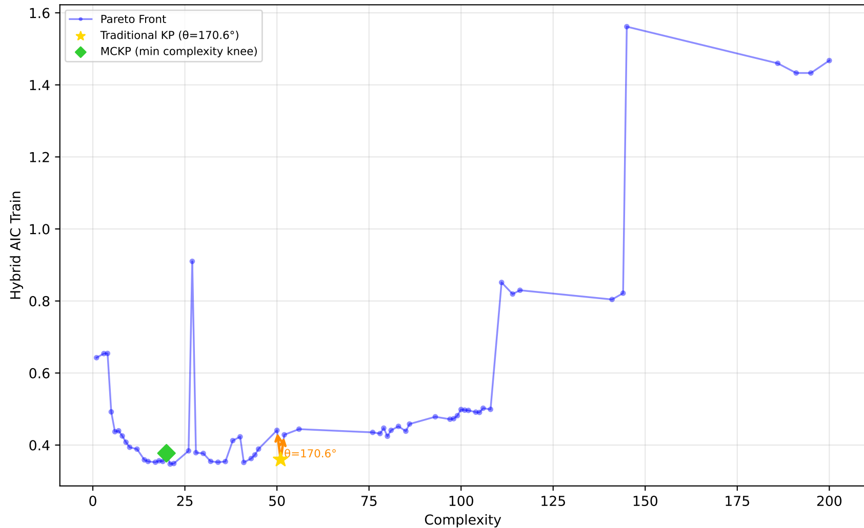
228_elusage - Run 30 - SVP - Hybrid AIC Train \lambda_1=0.60, \lambda_2=0.60, \lambda_3=1.00 | Difficulty: 0.45 | Method: mckp
