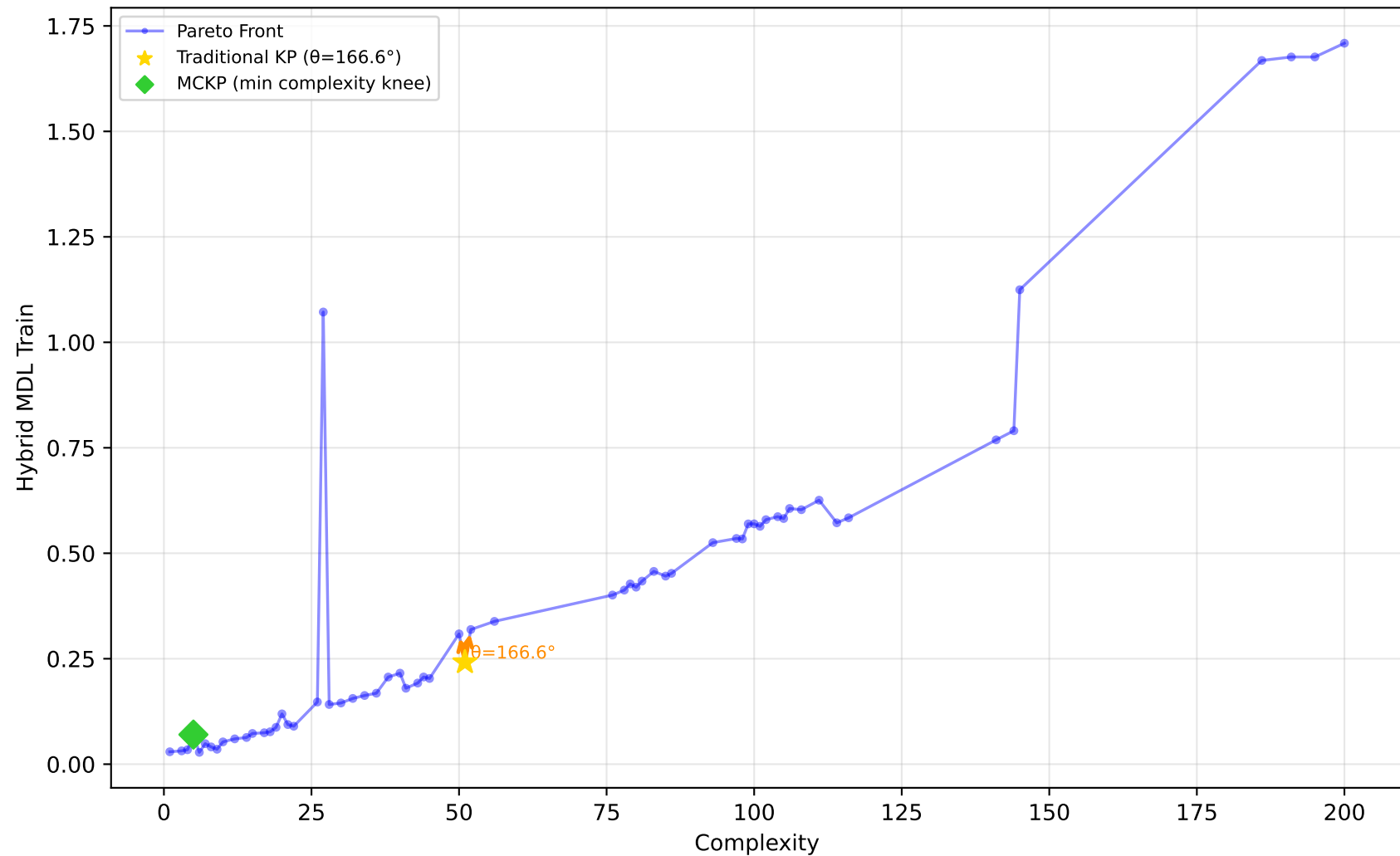
228_elusage - Run 30 - SVP - Hybrid MDL Train \lambda_1=0.00, \lambda_2=1.00, \lambda_3=0.00 | Difficulty: 0.45 | Method: mckp
