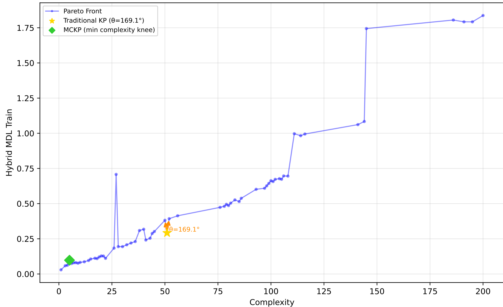
228_elusage - Run 30 - SVP - Hybrid MDL Train \lambda_1=0.60, \lambda_2=0.60, \lambda_3=1.00 | Difficulty: 0.45 | Method: mckp
