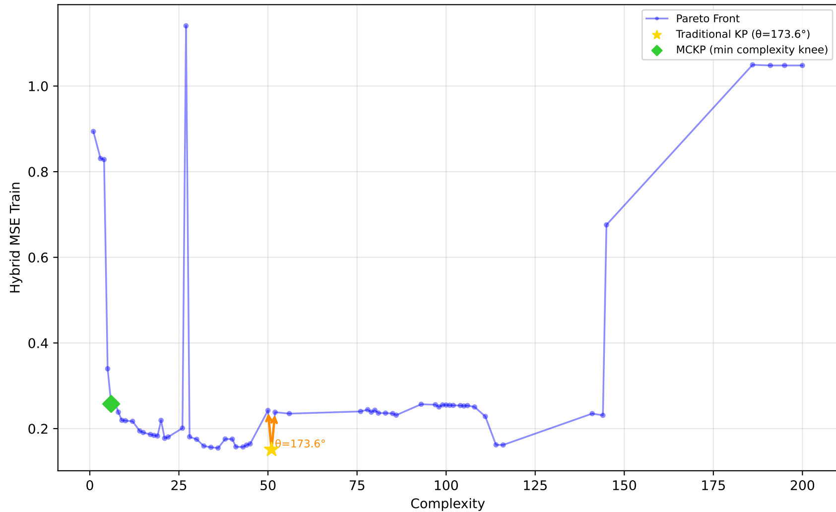
228_elusage - Run 30 - SVP - Hybrid MSE Train \lambda_1=0.00, \lambda_2=1.00, \lambda_3=0.00 | Difficulty: 0.45 | Method: mckp
