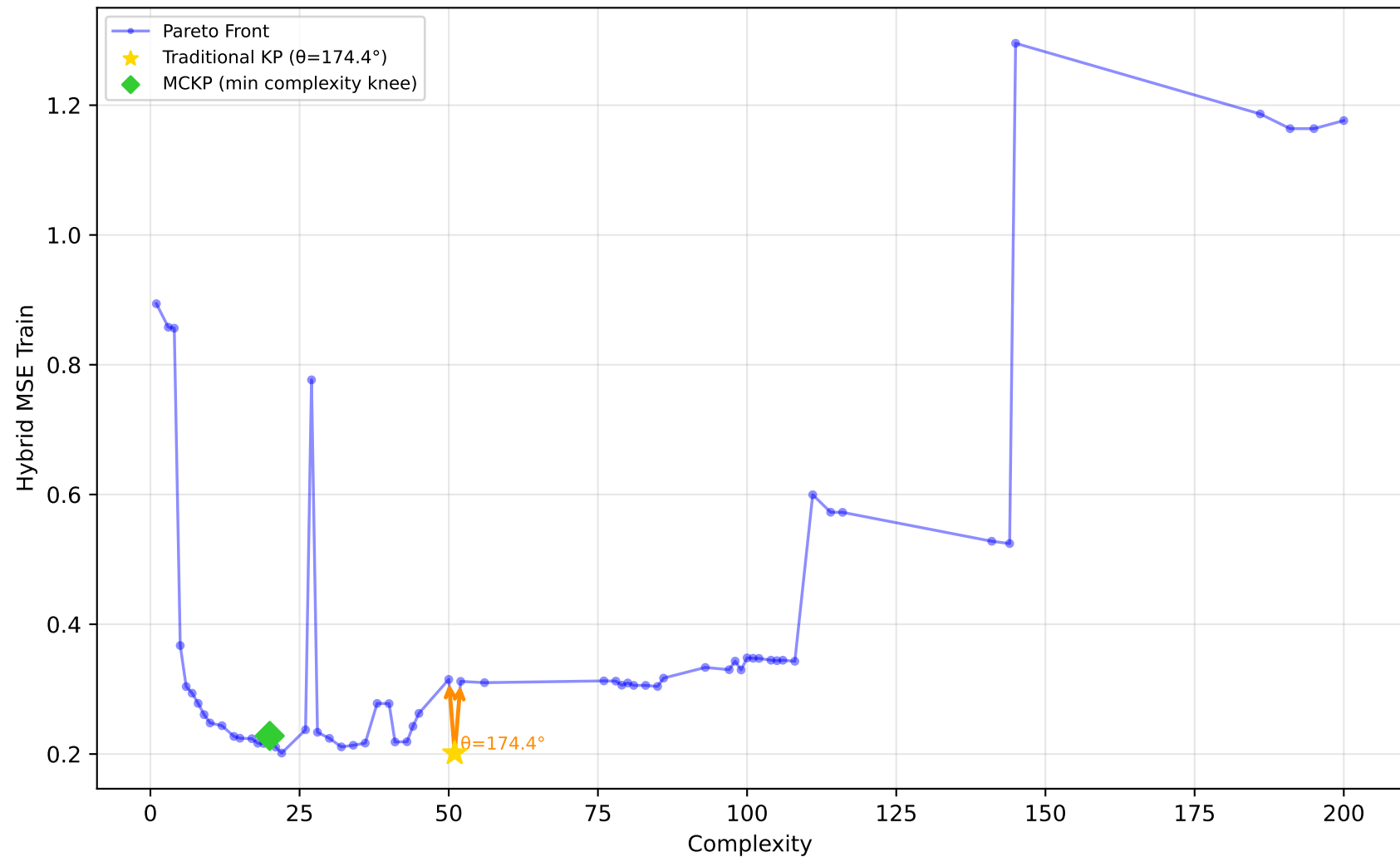
228_elusage - Run 30 - SVP - Hybrid MSE Train \lambda_1=0.60, \lambda_2=0.60, \lambda_3=1.00 | Difficulty: 0.45 | Method: mckp
