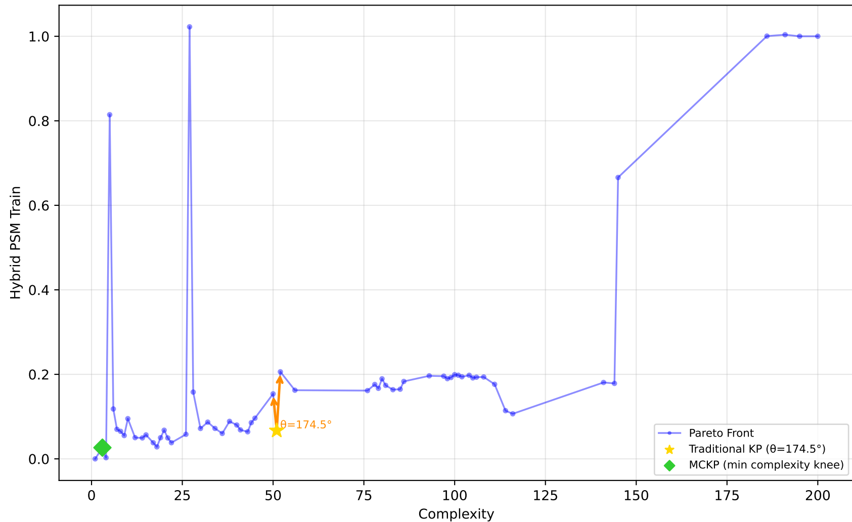
228_elusage - Run 30 - SVP - Hybrid PSM Train \lambda_1=0.00, \lambda_2=1.00, \lambda_3=0.00 | Difficulty: 0.45 | Method: mckp
