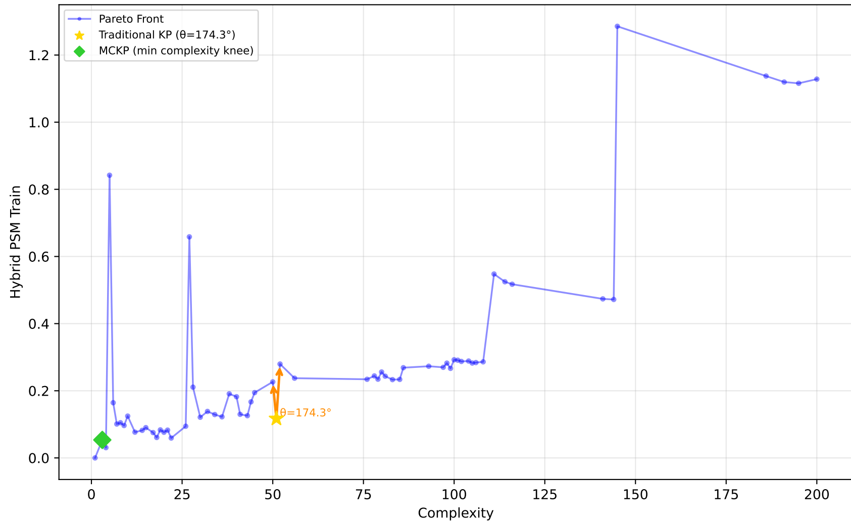
228_elusage - Run 30 - SVP - Hybrid PSM Train \lambda_1=0.60, \lambda_2=0.60, \lambda_3=1.00 | Difficulty: 0.45 | Method: mckp
