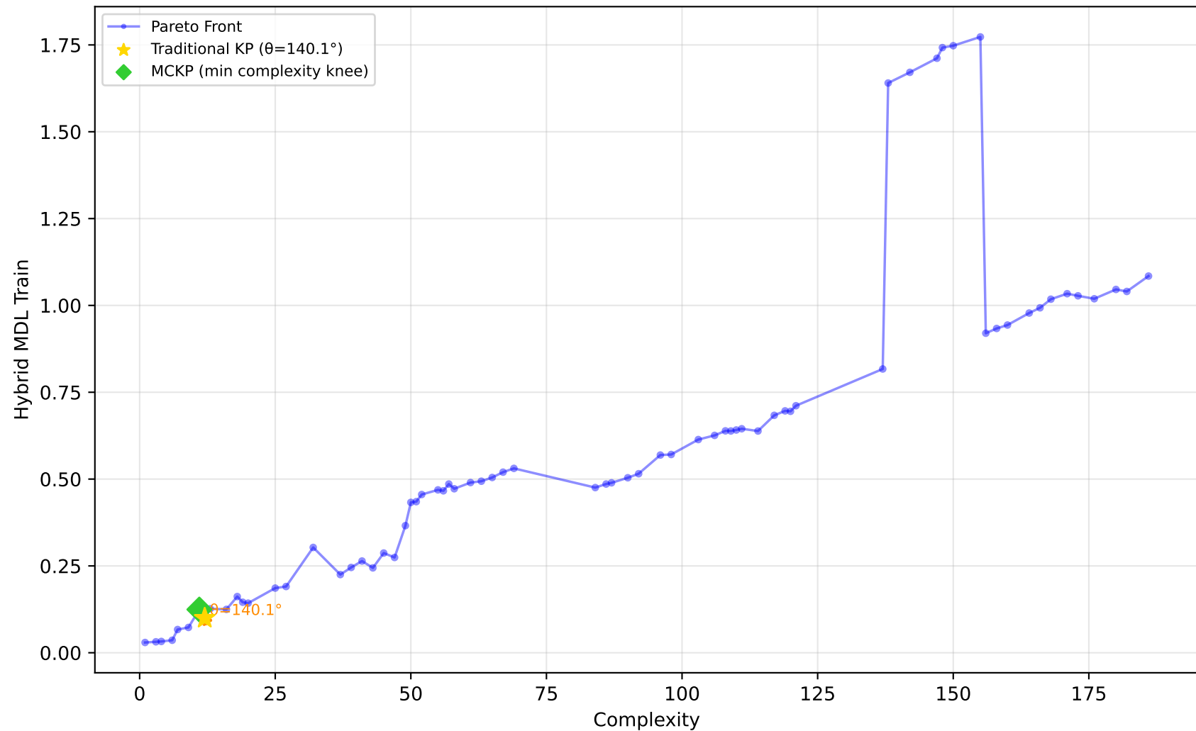
228_elusage - Run 3 - MVP - Hybrid MDL Train \lambda_1=0.00 , \lambda_2=0.00 , \lambda_3=1.00 | Difficulty: 1.00 | Method: hmr
