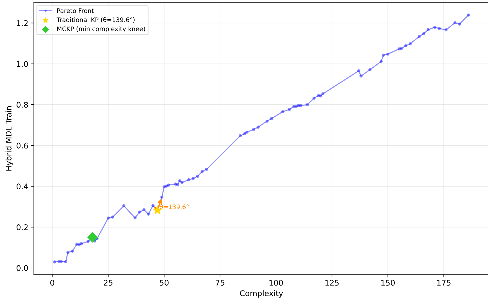
228_elusage - Run 3 - MVP - Hybrid MDL Train \lambda_1=0.00, \lambda_2=0.30, \lambda_3=0.00 | Difficulty: 1.00 | Method: hmr
