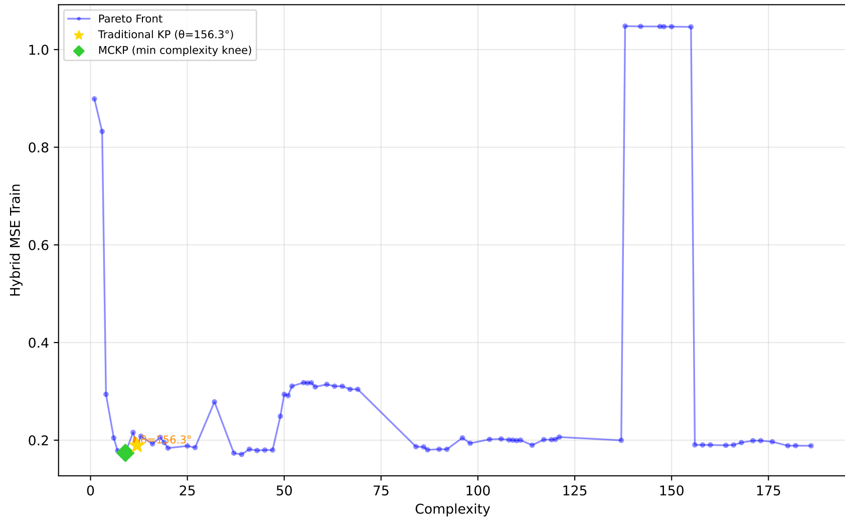
228_elusage - Run 3 - MVP - Hybrid MSE Train \lambda_1=0.00, \lambda_2=0.00, \lambda_3=1.00 | Difficulty: 1.00 | Method: hmr
