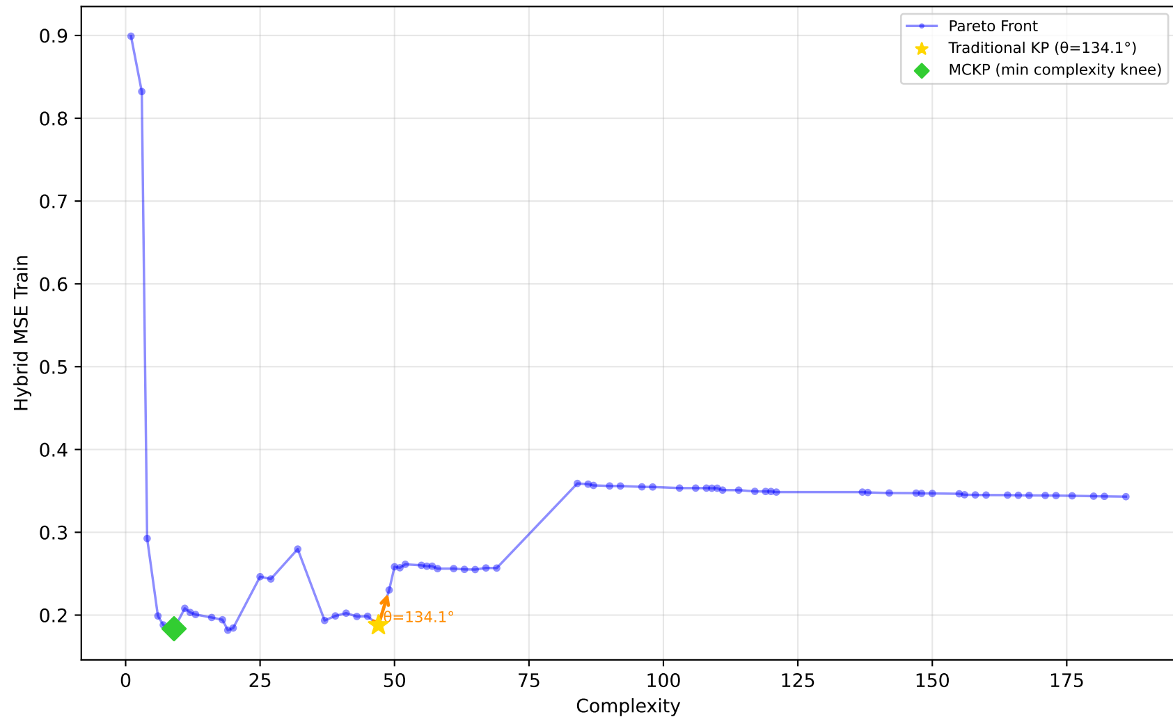
228_elusage - Run 3 - MVP - Hybrid MSE Train \lambda_1=0.00, \lambda_2=0.30, \lambda_3=0.00 | Difficulty: 1.00 | Method: hmr
