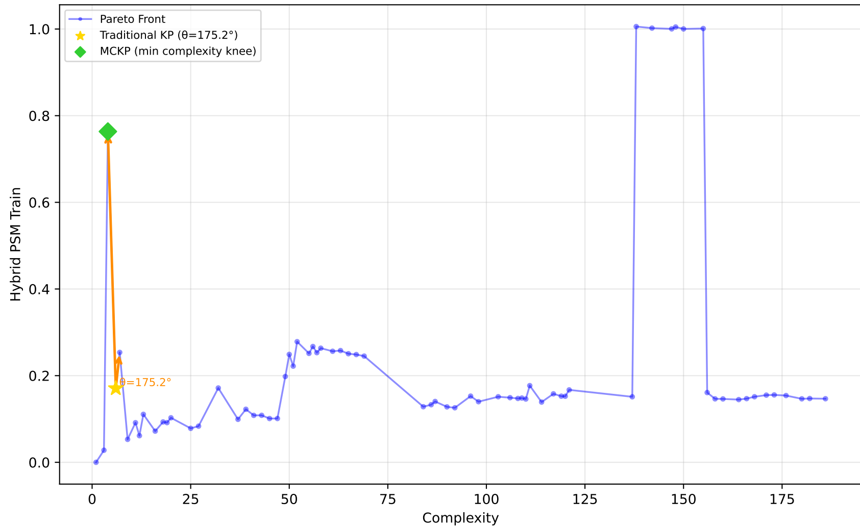
228_elusage - Run 3 - MVP - Hybrid PSM Train \lambda_1=0.00, \lambda_2=0.00, \lambda_3=1.00 | Difficulty: 1.00 | Method: hmr
