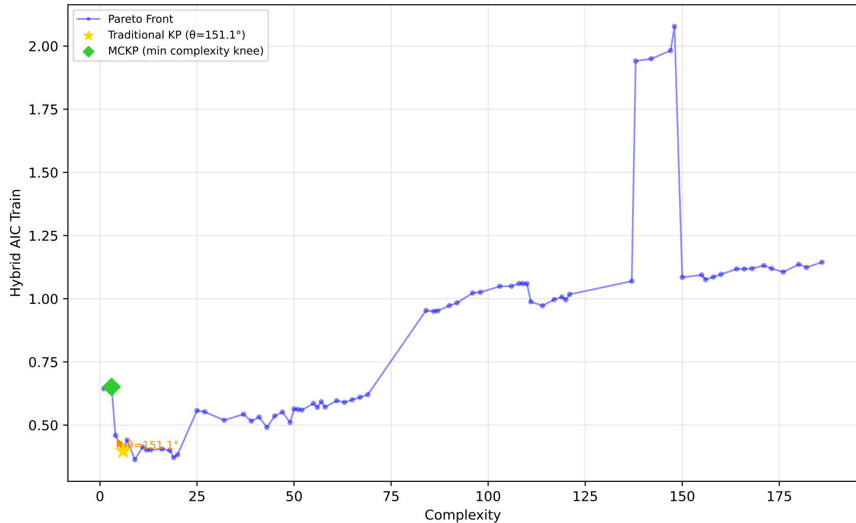
228_elusage - Run 3 - SVP - Hybrid AIC Train \lambda_1=0.60, \lambda_2=0.60, \lambda_3=1.00 | Difficulty: 1.00 | Method: hmr
