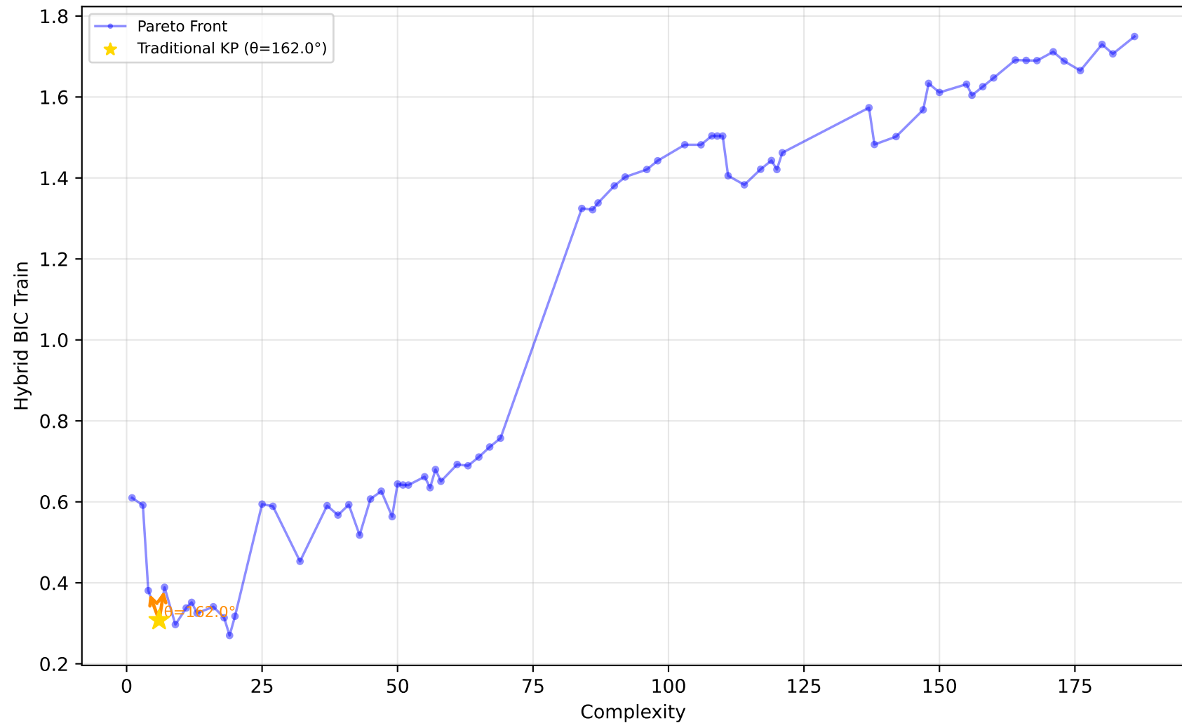
228_elusage - Run 3 - SVP - Hybrid BIC Train \lambda_1=0.00, \lambda_2=1.00, \lambda_3=0.00 | Difficulty: 1.00 | Method: hmr
