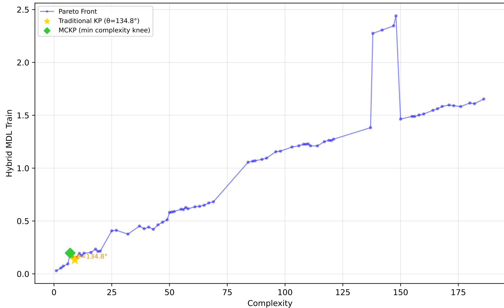
228_elusage - Run 3 - SVP - Hybrid MDL Train \lambda_1=0.60, \lambda_2=0.60, \lambda_3=1.00 | Difficulty: 1.00 | Method: hmr
