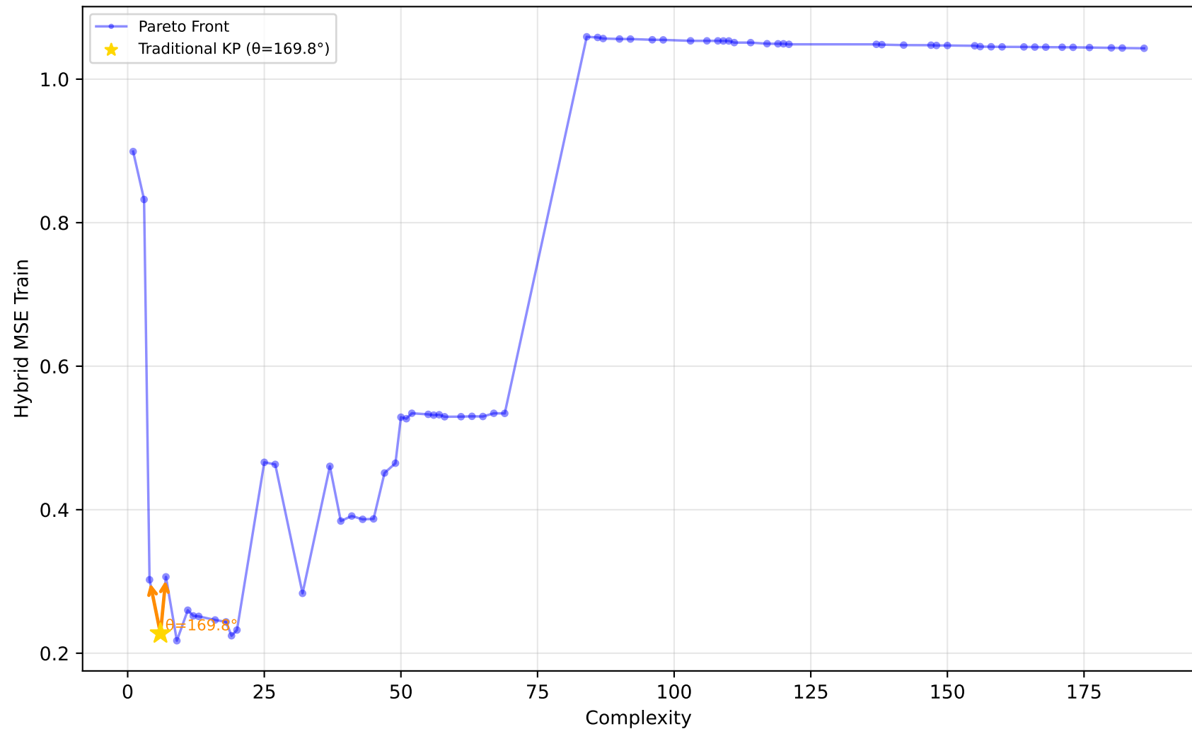
228_elusage - Run 3 - SVP - Hybrid MSE Train \lambda_1=0.00, \lambda_2=1.00, \lambda_3=0.00 | Difficulty: 1.00 | Method: hmr
