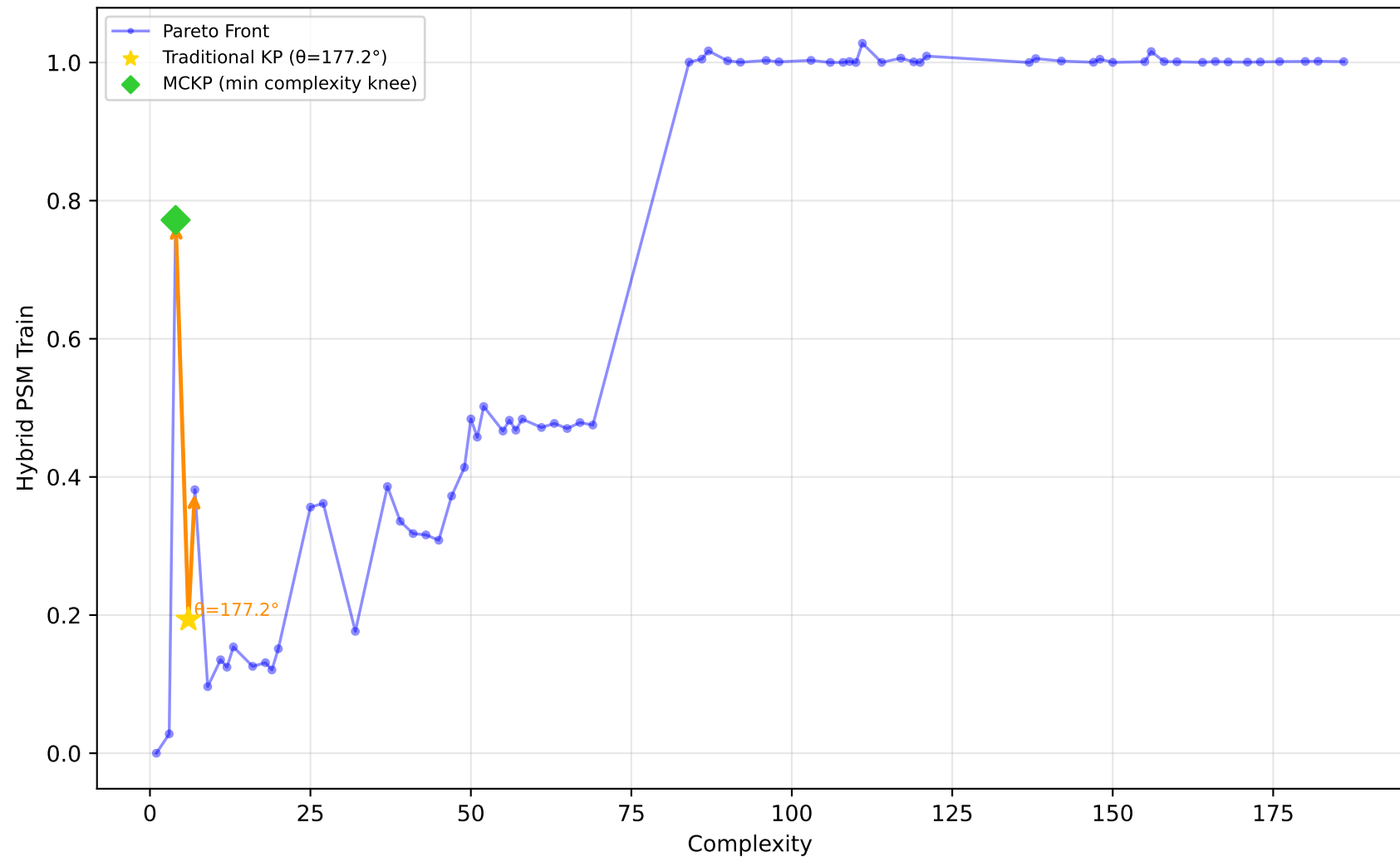
228_elusage - Run 3 - SVP - Hybrid PSM Train \lambda_1=0.00, \lambda_2=1.00, \lambda_3=0.00 | Difficulty: 1.00 | Method: hmr
