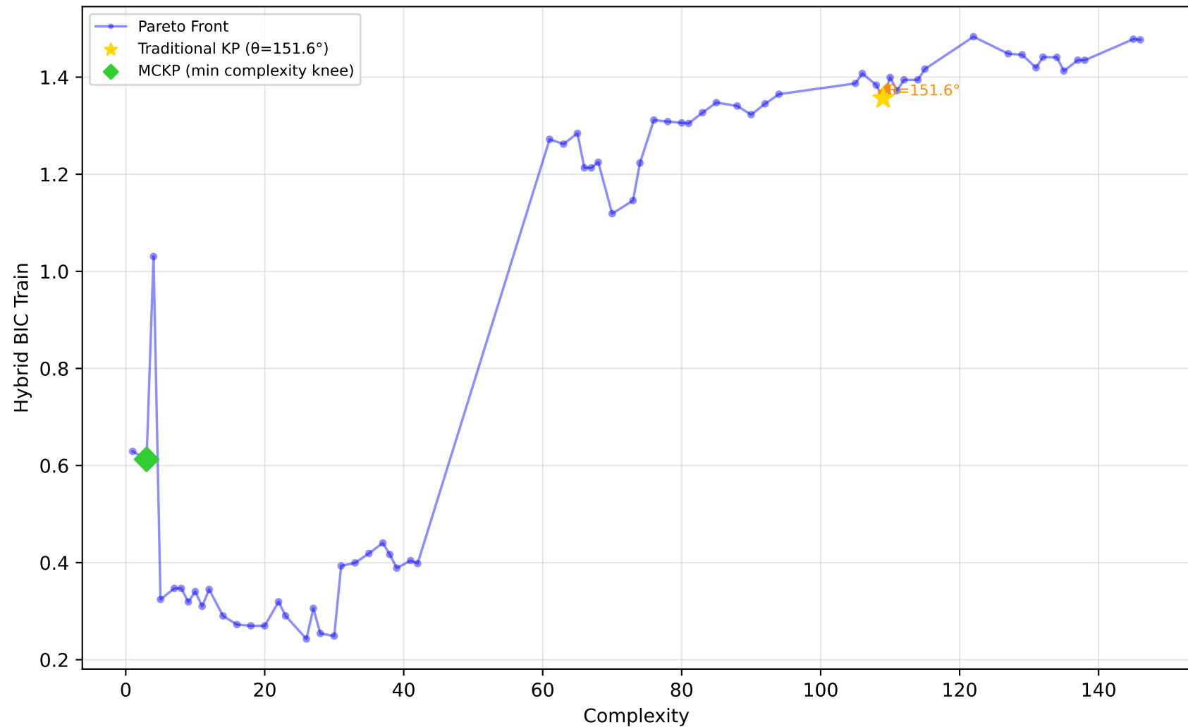
228_elusage - Run 4 - MVP - Hybrid BIC Train \lambda_1=0.00, \lambda_2=0.00, \lambda_3=1.00 | Difficulty: 0.48 | Method: mckp
