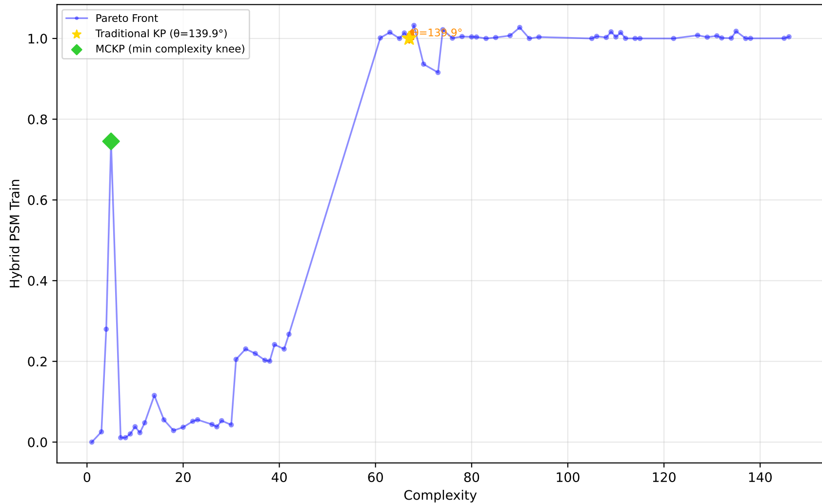
228_elusage - Run 4 - MVP - Hybrid PSM Train \lambda_1=0.00, \lambda_2=0.00, \lambda_3=1.00 | Difficulty: 0.48 | Method: mckp
