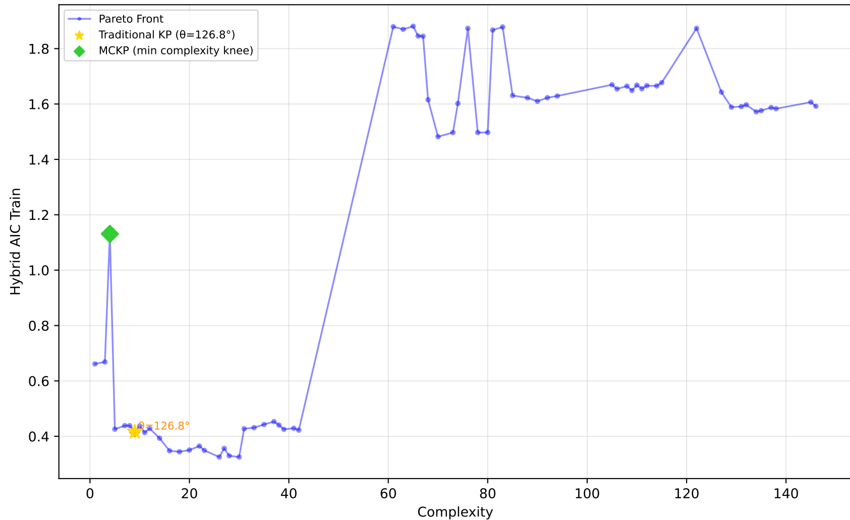
228_elusage - Run 4 - SVP - Hybrid AIC Train \lambda_1=0.60, \lambda_2=0.60, \lambda_3=1.00 | Difficulty: 0.48 | Method: mckp
