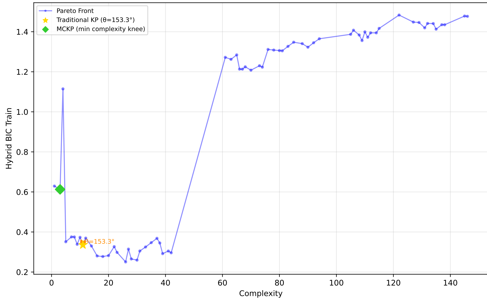
228_elusage - Run 4 - SVP - Hybrid BIC Train \lambda_1=0.00, \lambda_2=1.00, \lambda_3=0.00 | Difficulty: 0.48 | Method: mckp
