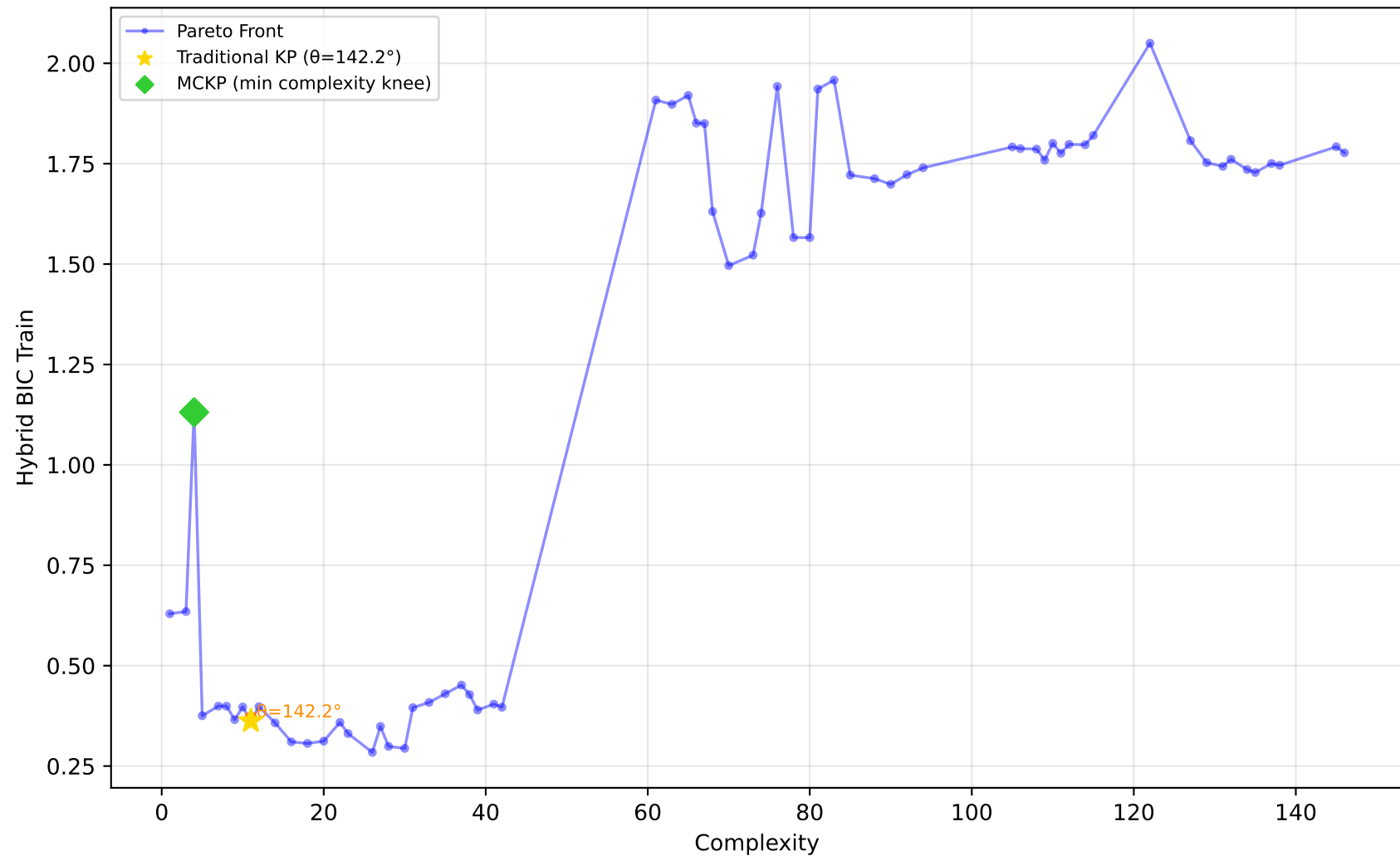
228_elusage - Run 4 - SVP - Hybrid BIC Train \lambda_1=0.60, \lambda_2=0.60, \lambda_3=1.00 | Difficulty: 0.48 | Method: mckp
