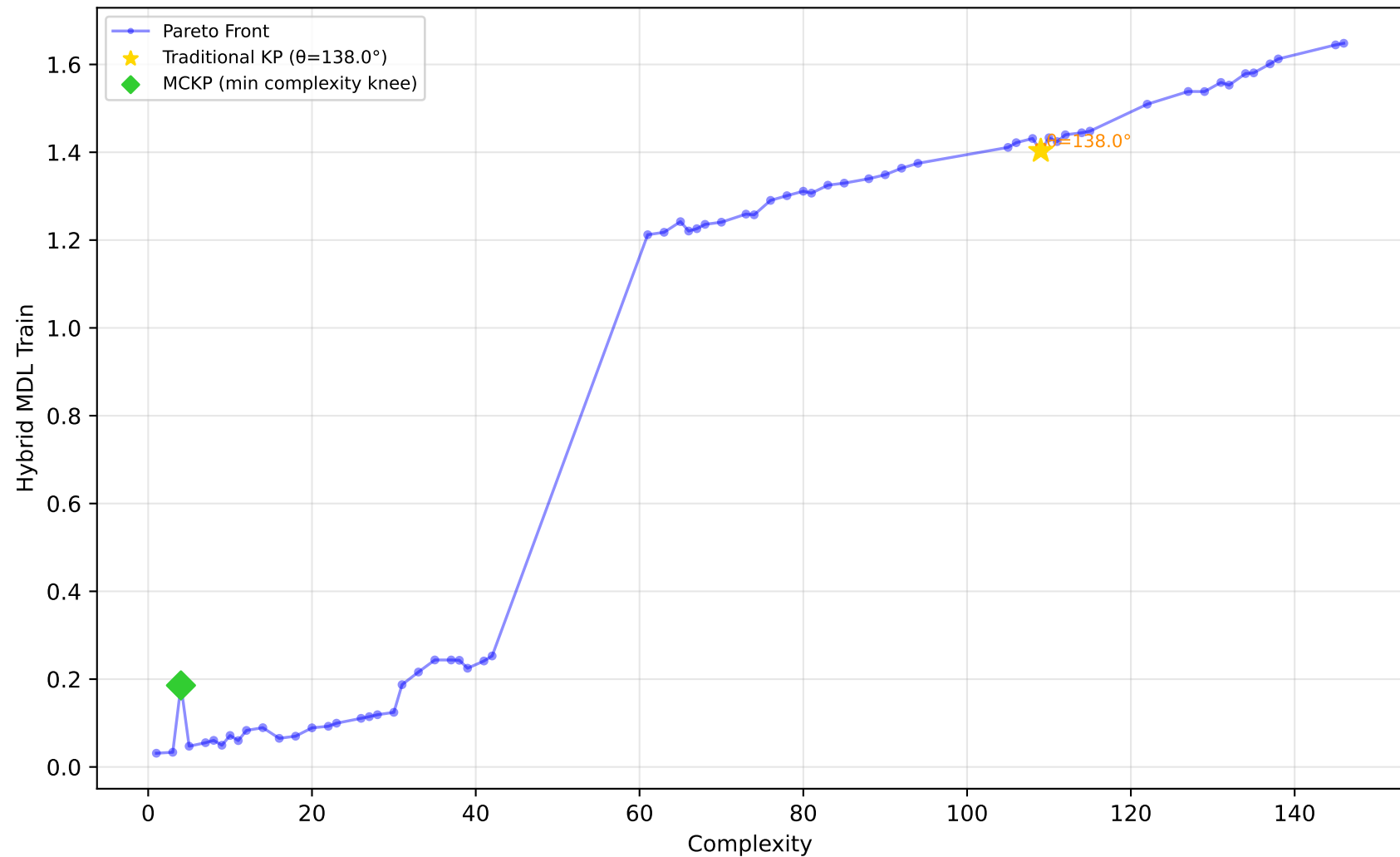
228_elusage - Run 4 - SVP - Hybrid MDL Train \lambda_1=0.00 , \lambda_2=1.00 , \lambda_3=0.00 | Difficulty: 0.48 | Method: mckp
