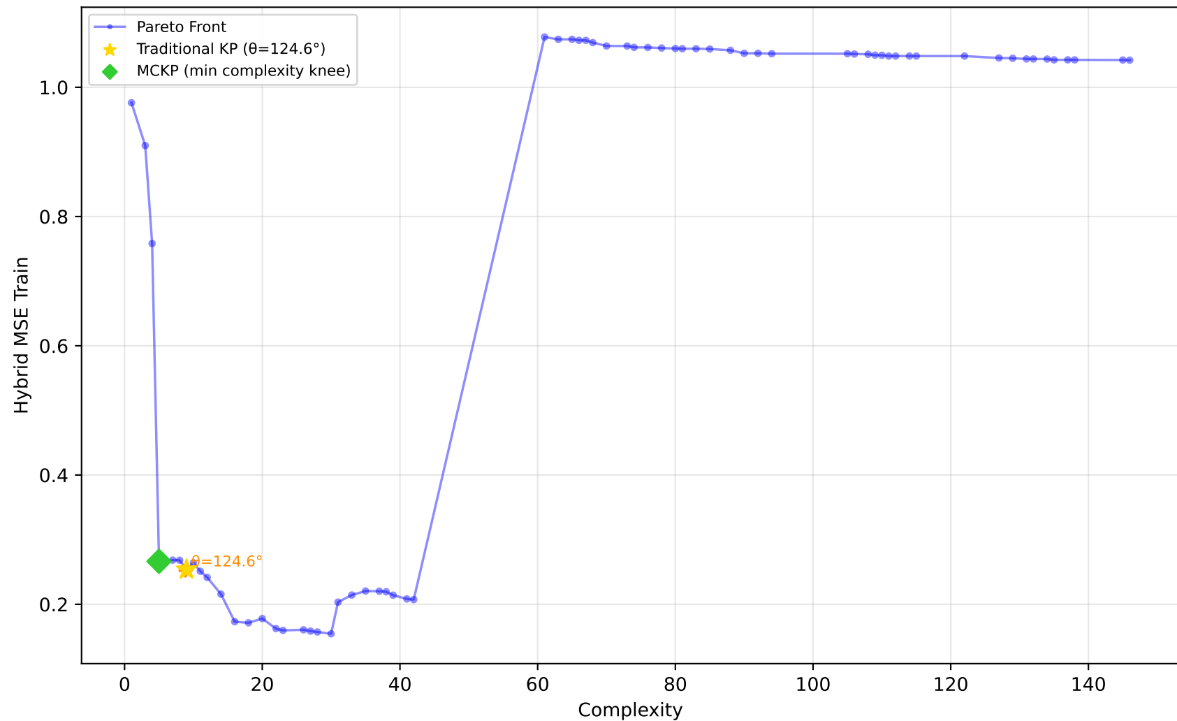
228_elusage - Run 4 - SVP - Hybrid MSE Train \lambda_1=0.00, \lambda_2=1.00, \lambda_3=0.00 | Difficulty: 0.48 | Method: mckp
