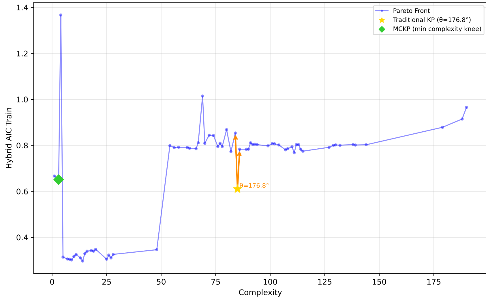
228_elusage - Run 5 - MVP - Hybrid AIC Train \lambda_1=0.00, \lambda_2=0.00, \lambda_3=1.00 | Difficulty: 0.25 | Method: mckp
