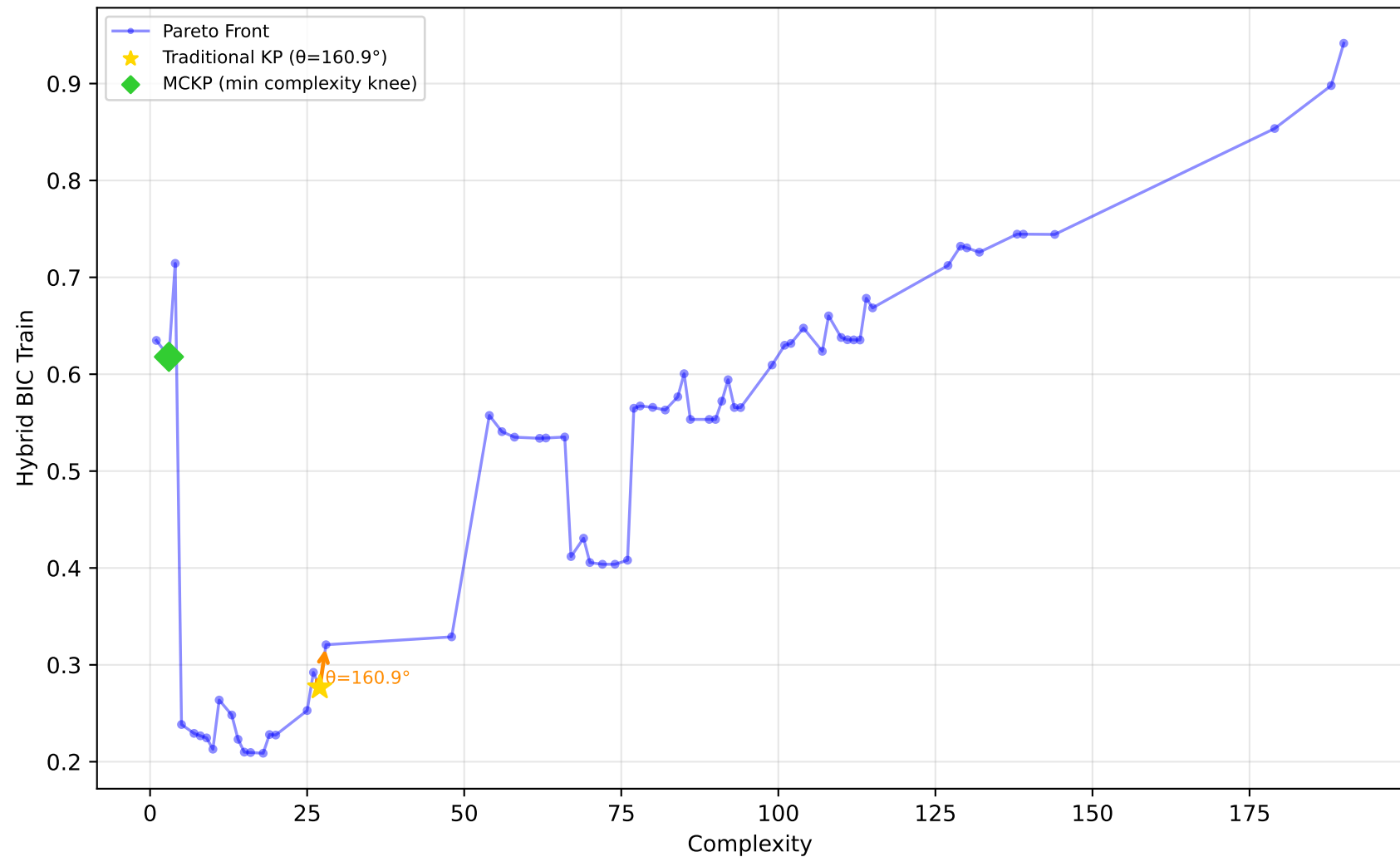
228_elusage - Run 5 - MVP - Hybrid BIC Train \lambda_1=0.00, \lambda_2=0.30, \lambda_3=0.00 | Difficulty: 0.25 | Method: mckp
