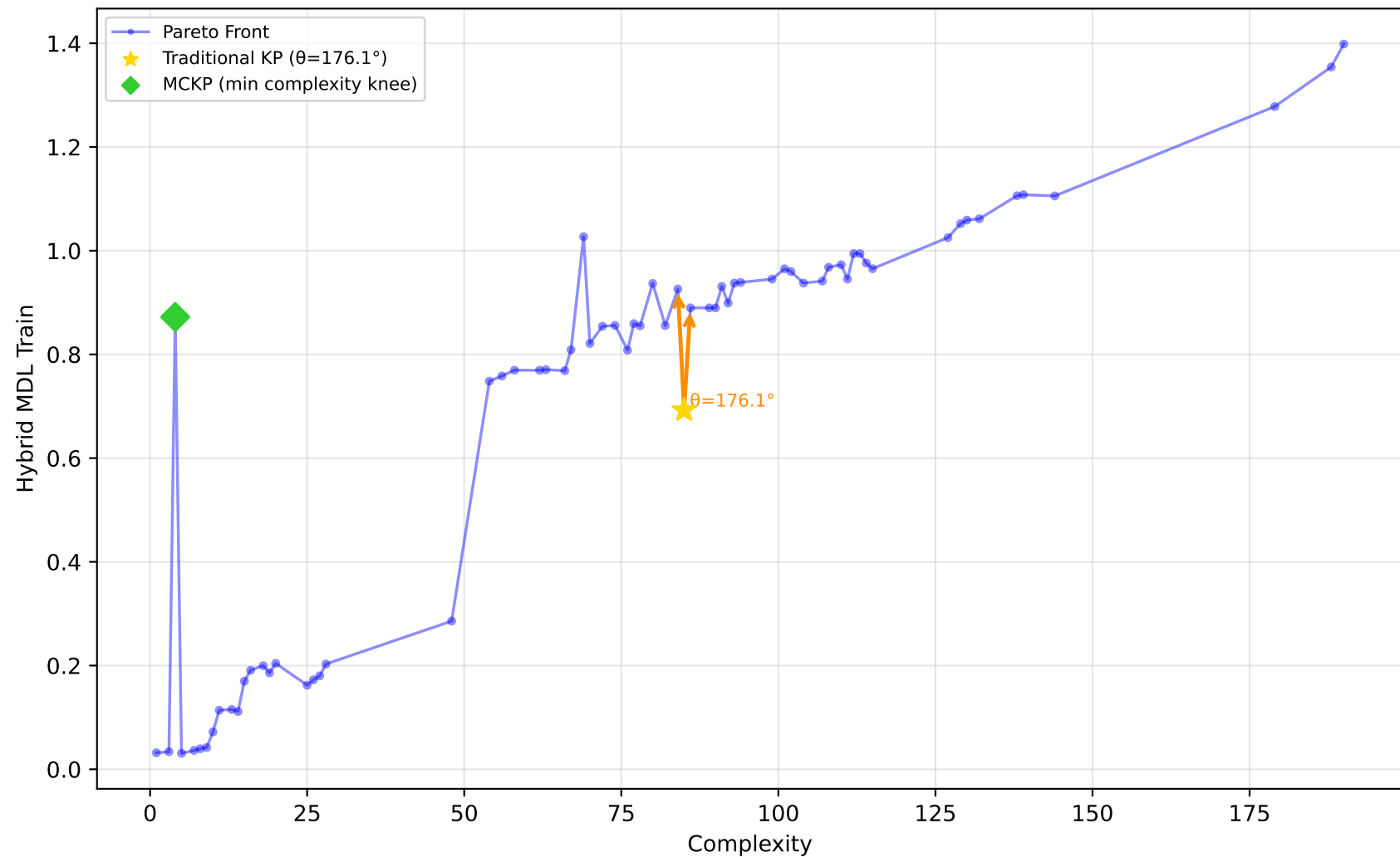
228_elusage - Run 5 - MVP - Hybrid MDL Train \lambda_1=0.00, \lambda_2=0.00, \lambda_3=1.00 | Difficulty: 0.25 | Method: mckp
