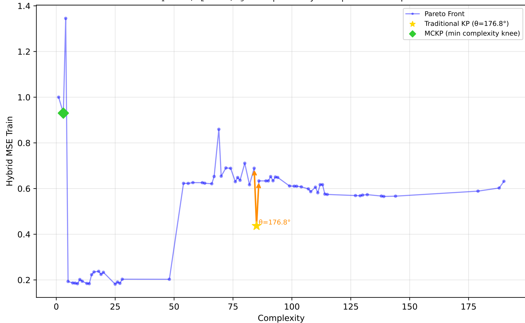
228_elusage - Run 5 - MVP - Hybrid MSE Train \lambda_1=0.00, \lambda_2=0.00, \lambda_3=1.00 | Difficulty: 0.25 | Method: mckp
