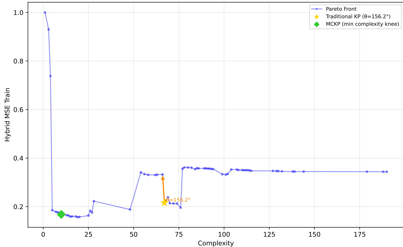
228_elusage - Run 5 - MVP - Hybrid MSE Train \lambda_1=0.00, \lambda_2=0.30, \lambda_3=0.00 | Difficulty: 0.25 | Method: mckp
