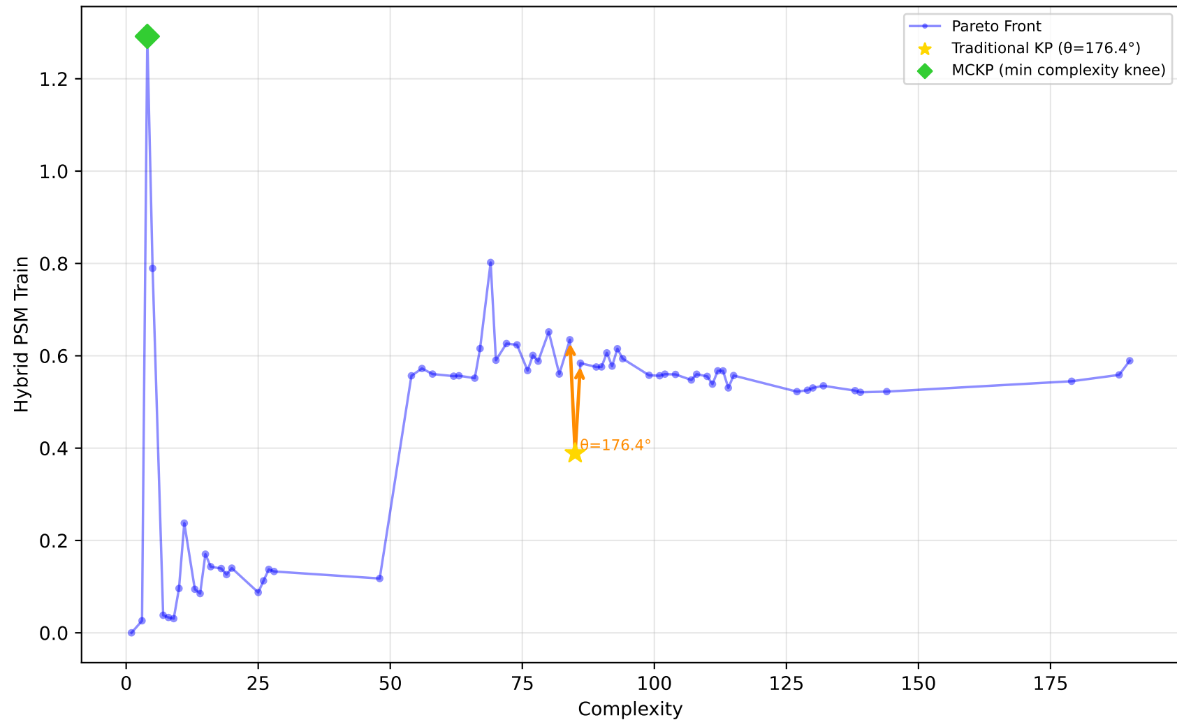
228_elusage - Run 5 - MVP - Hybrid PSM Train \lambda_1=0.00, \lambda_2=0.00, \lambda_3=1.00 | Difficulty: 0.25 | Method: mckp
