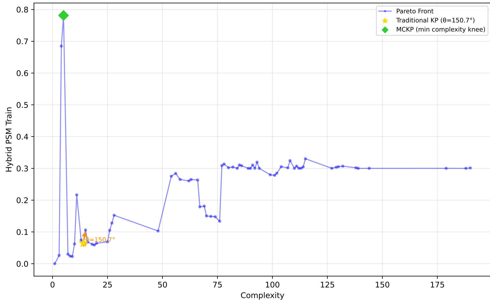
228_elusage - Run 5 - MVP - Hybrid PSM Train \lambda_1=0.00, \lambda_2=0.30, \lambda_3=0.00 | Difficulty: 0.25 | Method: mckp
