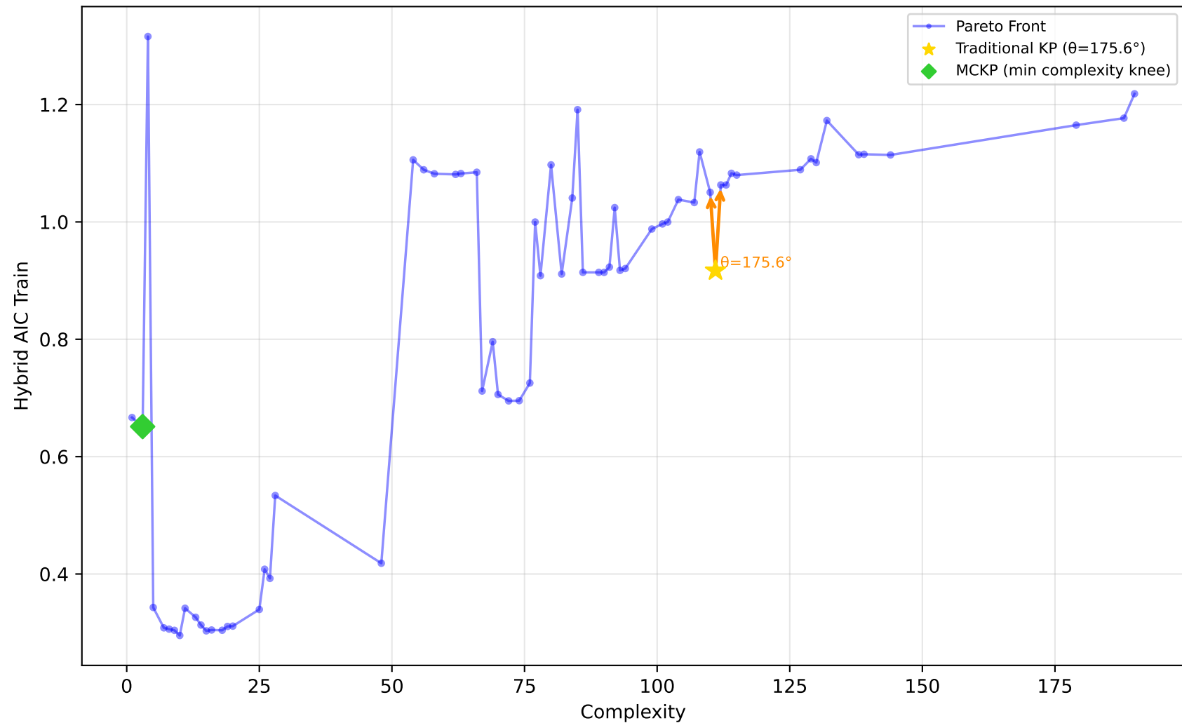
228_elusage - Run 5 - SVP - Hybrid AIC Train \lambda_1=0.00, \lambda_2=1.00, \lambda_3=0.00 | Difficulty: 0.25 | Method: mckp
