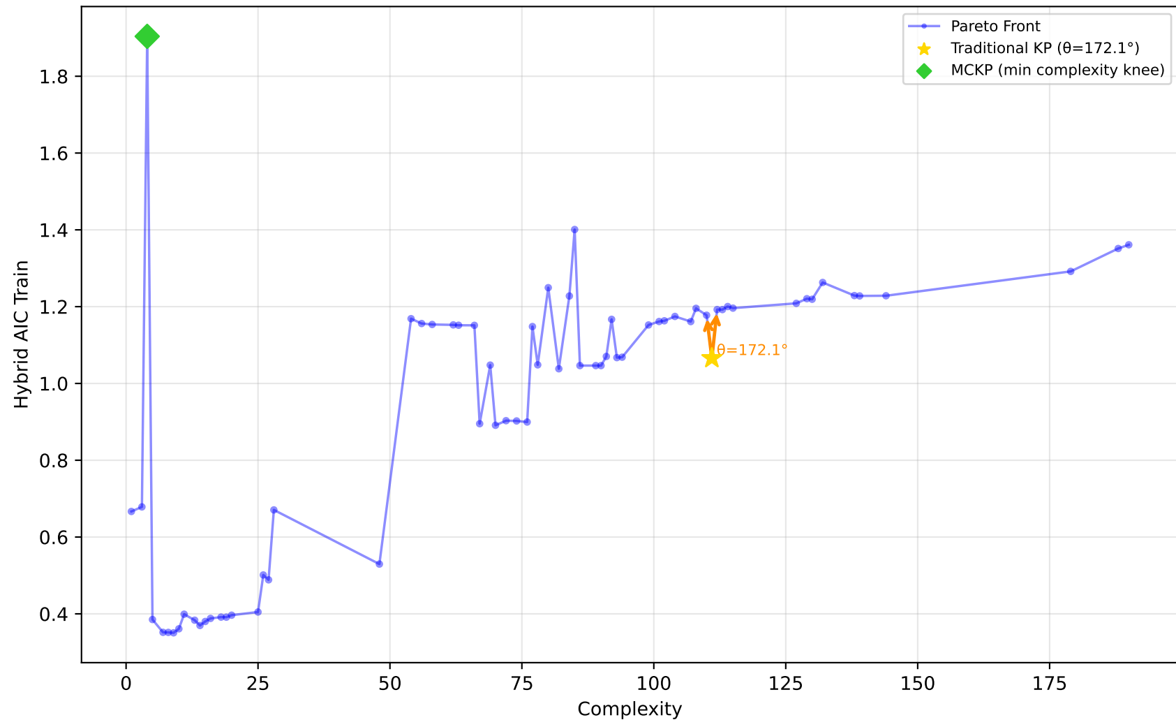
228_elusage - Run 5 - SVP - Hybrid AIC Train \lambda_1=0.60, \lambda_2=0.60, \lambda_3=1.00 | Difficulty: 0.25 | Method: mckp
