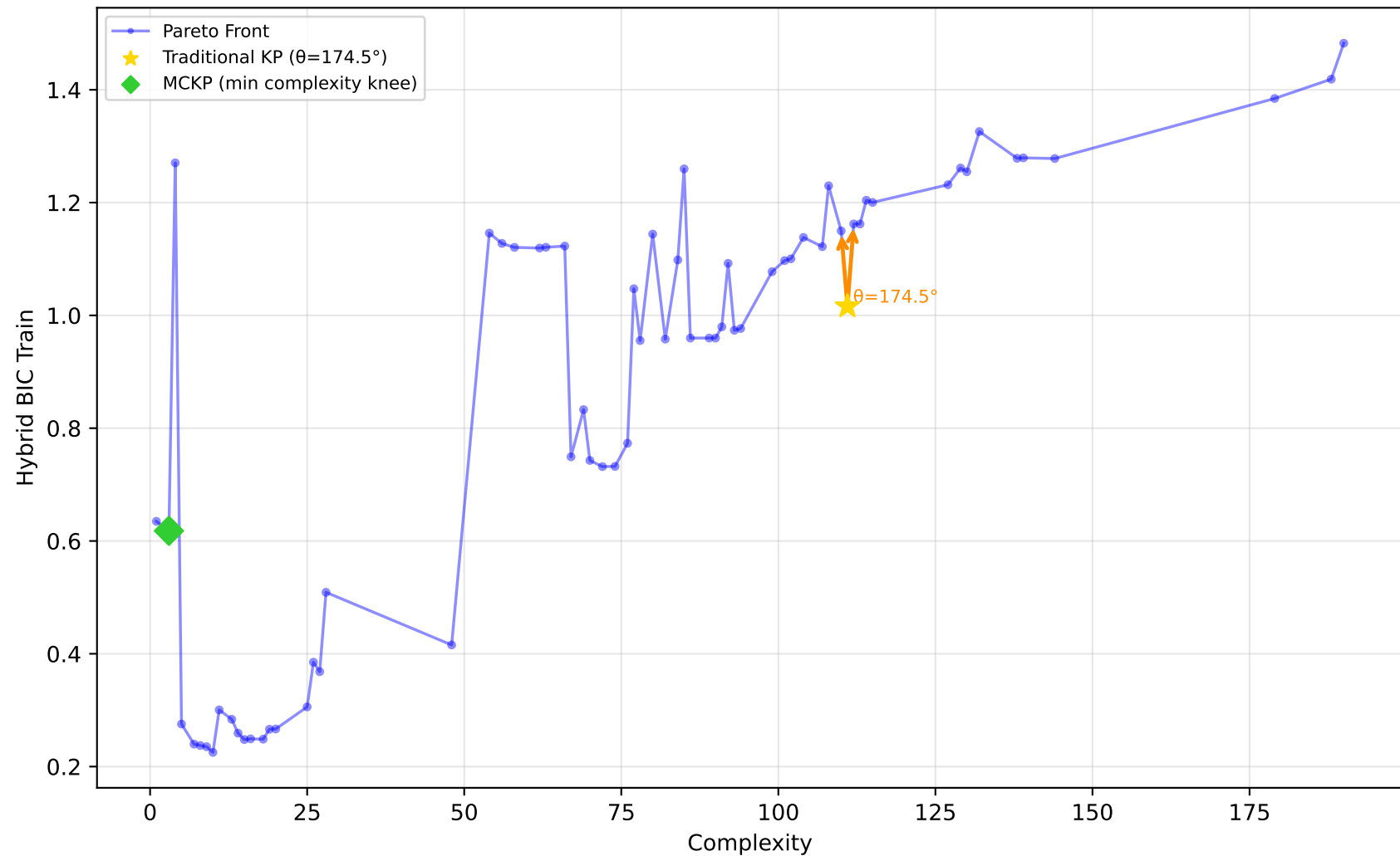
228_elusage - Run 5 - SVP - Hybrid BIC Train \lambda_1=0.00, \lambda_2=1.00, \lambda_3=0.00 | Difficulty: 0.25 | Method: mckp
