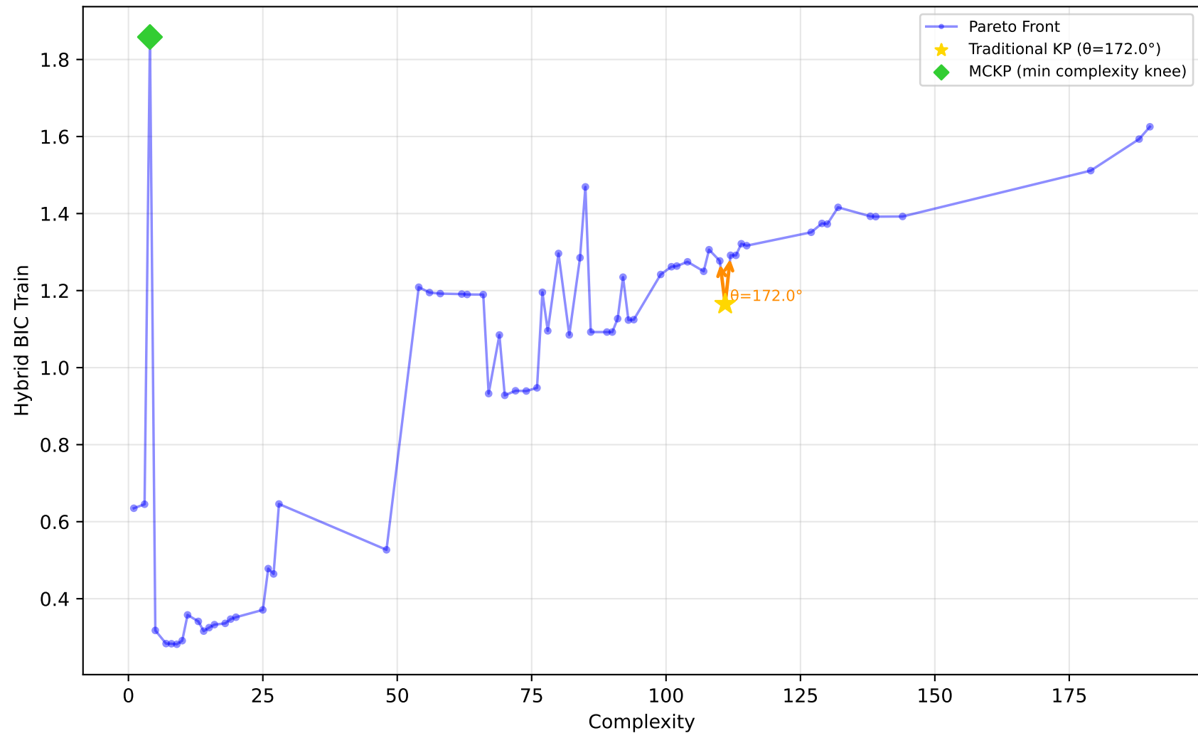
228_elusage - Run 5 - SVP - Hybrid BIC Train \lambda_1=0.60, \lambda_2=0.60, \lambda_3=1.00 | Difficulty: 0.25 | Method: mckp
