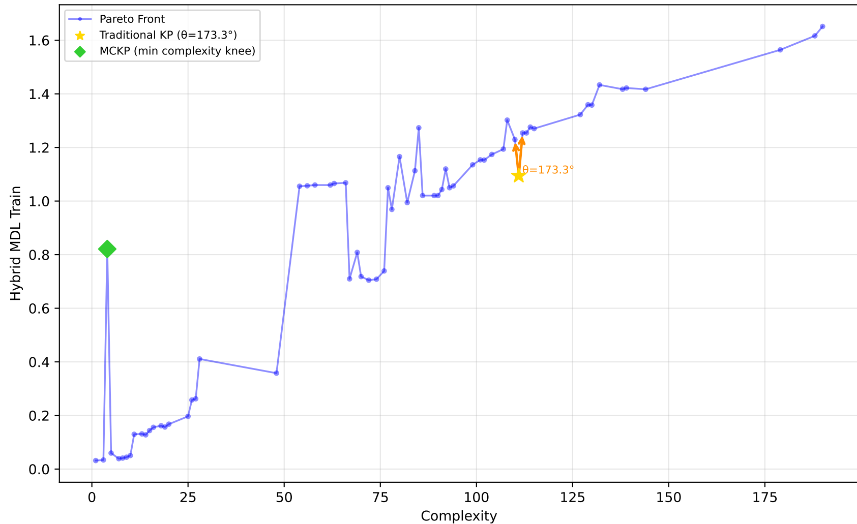
228_elusage - Run 5 - SVP - Hybrid MDL Train \lambda_1=0.00, \lambda_2=1.00, \lambda_3=0.00 | Difficulty: 0.25 | Method: mckp
