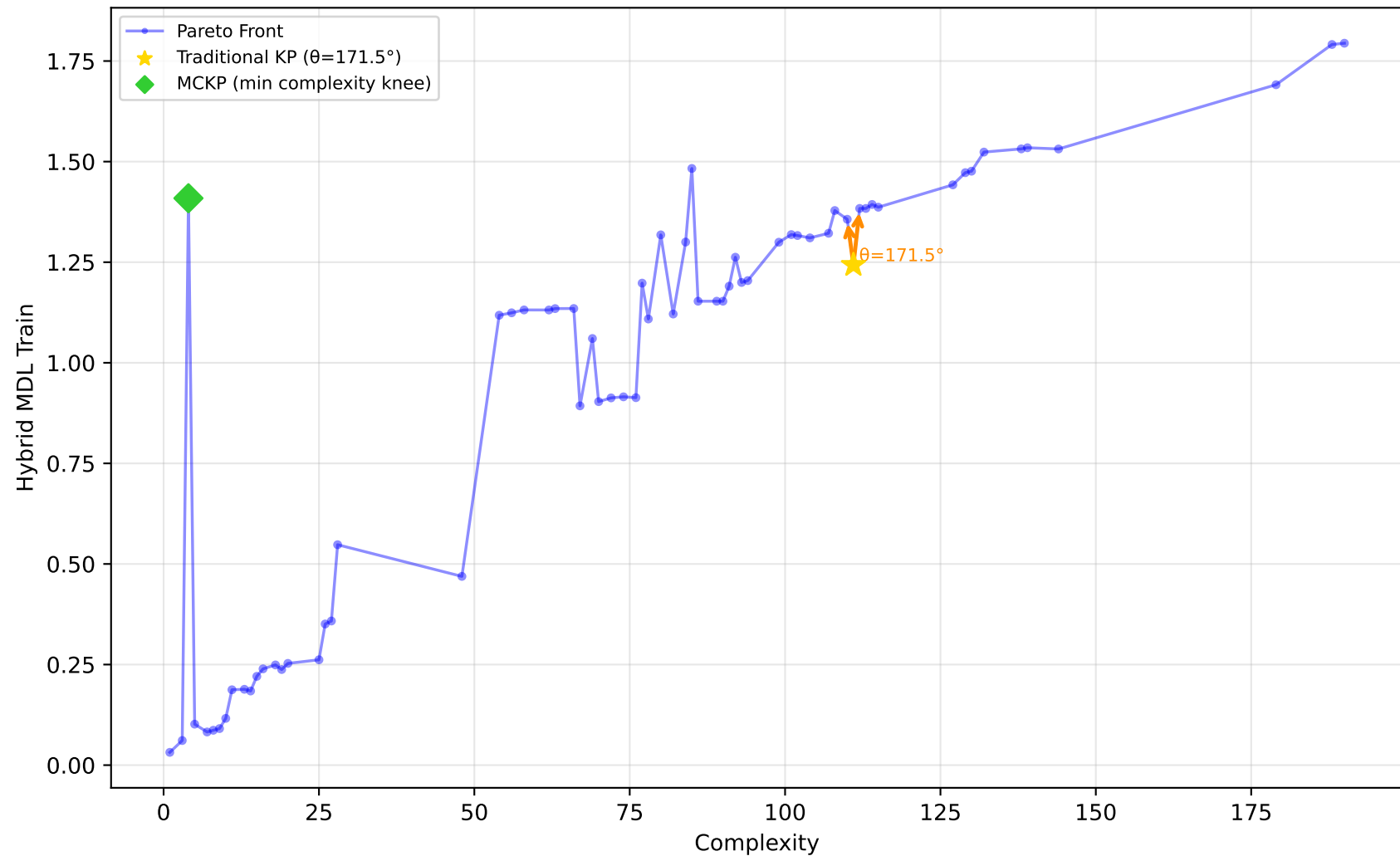
228_elusage - Run 5 - SVP - Hybrid MDL Train \lambda_1=0.60, \lambda_2=0.60, \lambda_3=1.00 | Difficulty: 0.25 | Method: mckp
