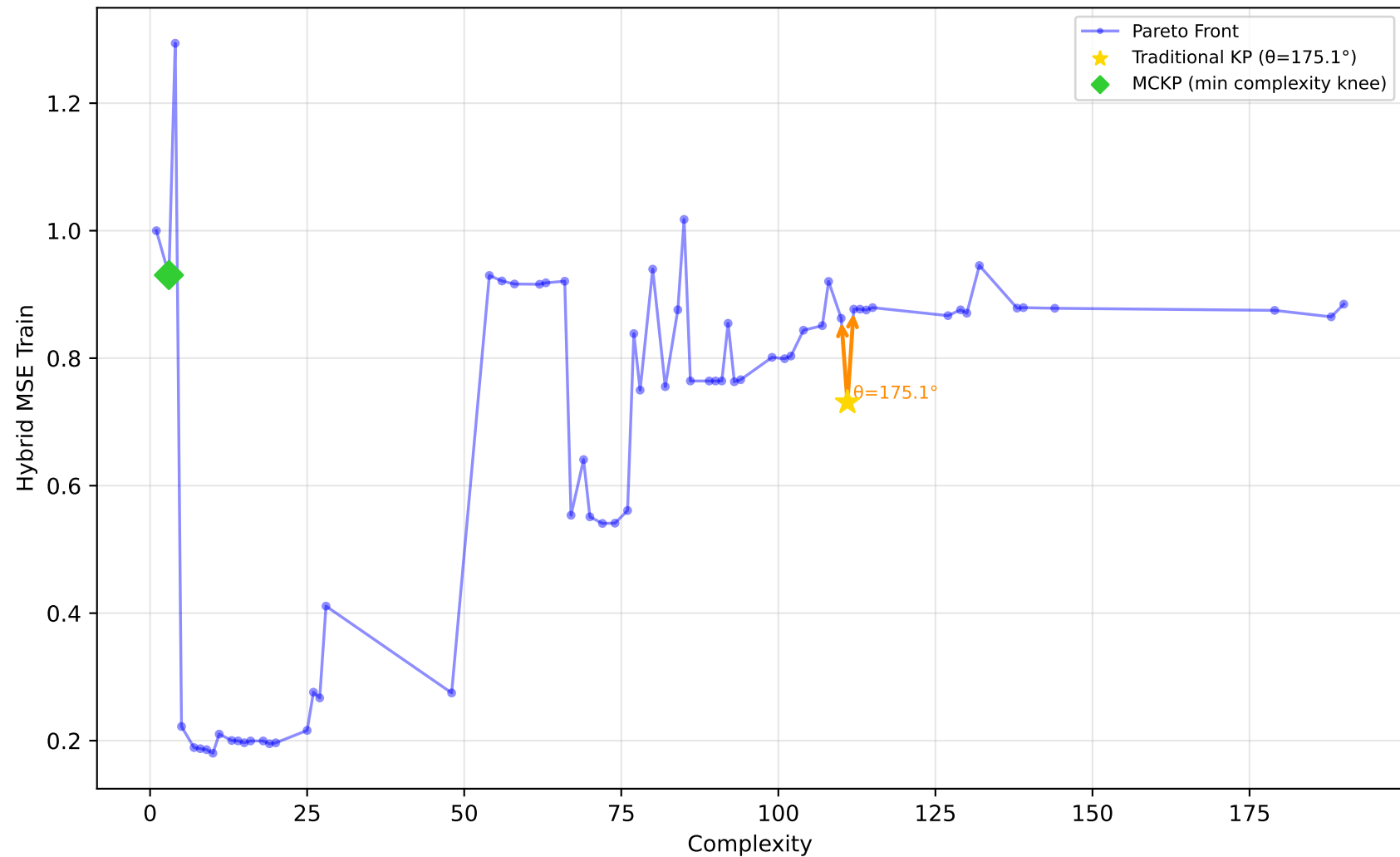
228_elusage - Run 5 - SVP - Hybrid MSE Train \lambda_1=0.00, \lambda_2=1.00, \lambda_3=0.00 | Difficulty: 0.25 | Method: mckp
