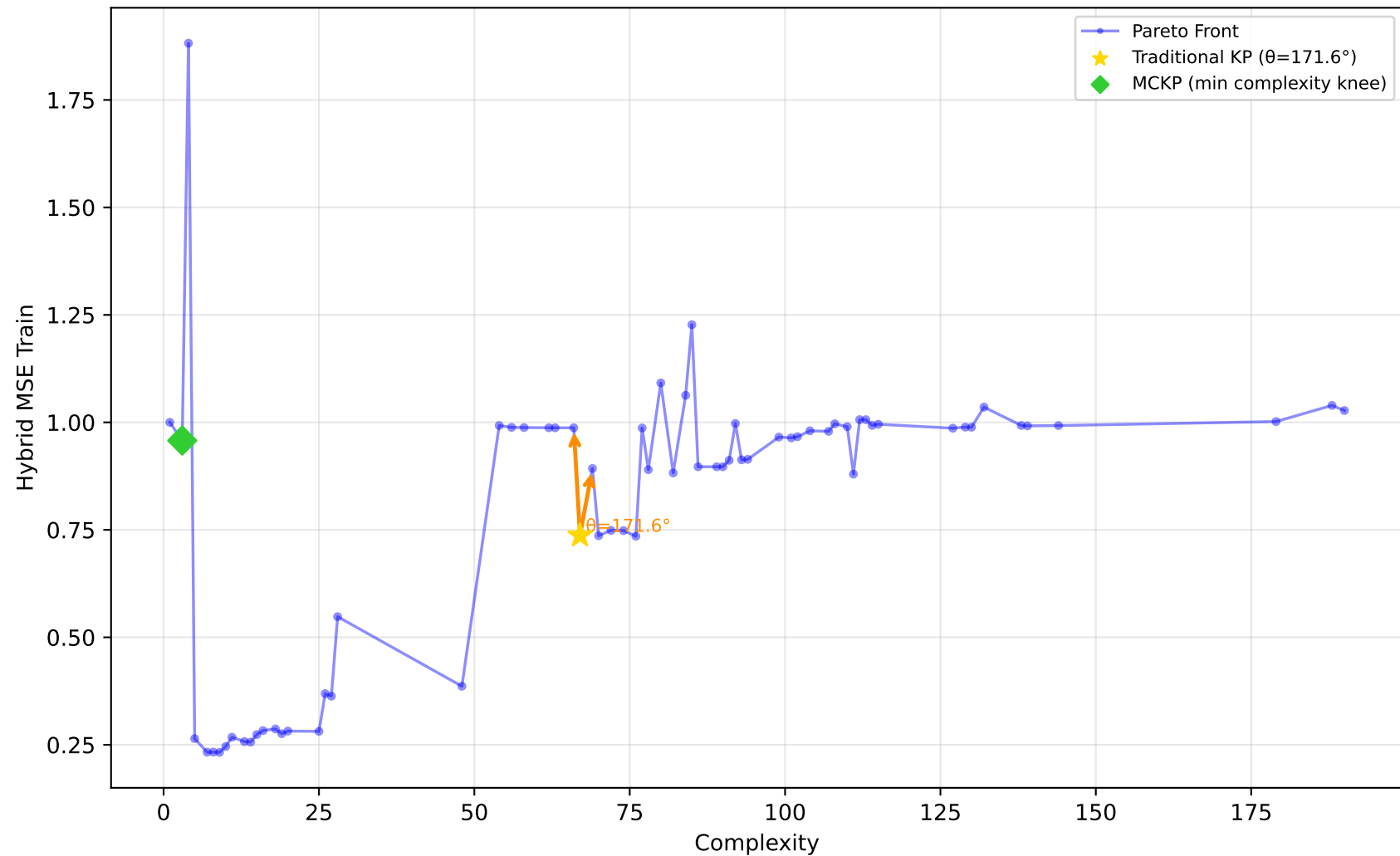
228_elusage - Run 5 - SVP - Hybrid MSE Train \lambda_1=0.60, \lambda_2=0.60, \lambda_3=1.00 | Difficulty: 0.25 | Method: mckp
