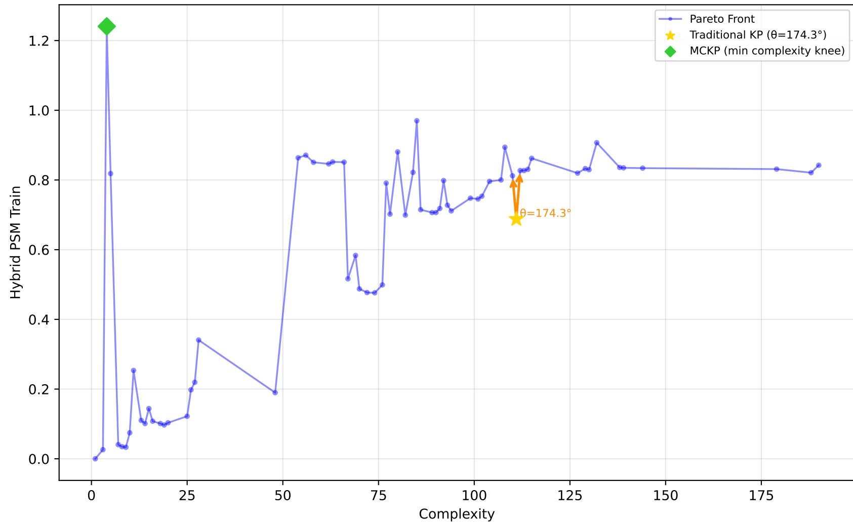
228_elusage - Run 5 - SVP - Hybrid PSM Train \lambda_1=0.00, \lambda_2=1.00, \lambda_3=0.00 | Difficulty: 0.25 | Method: mckp
