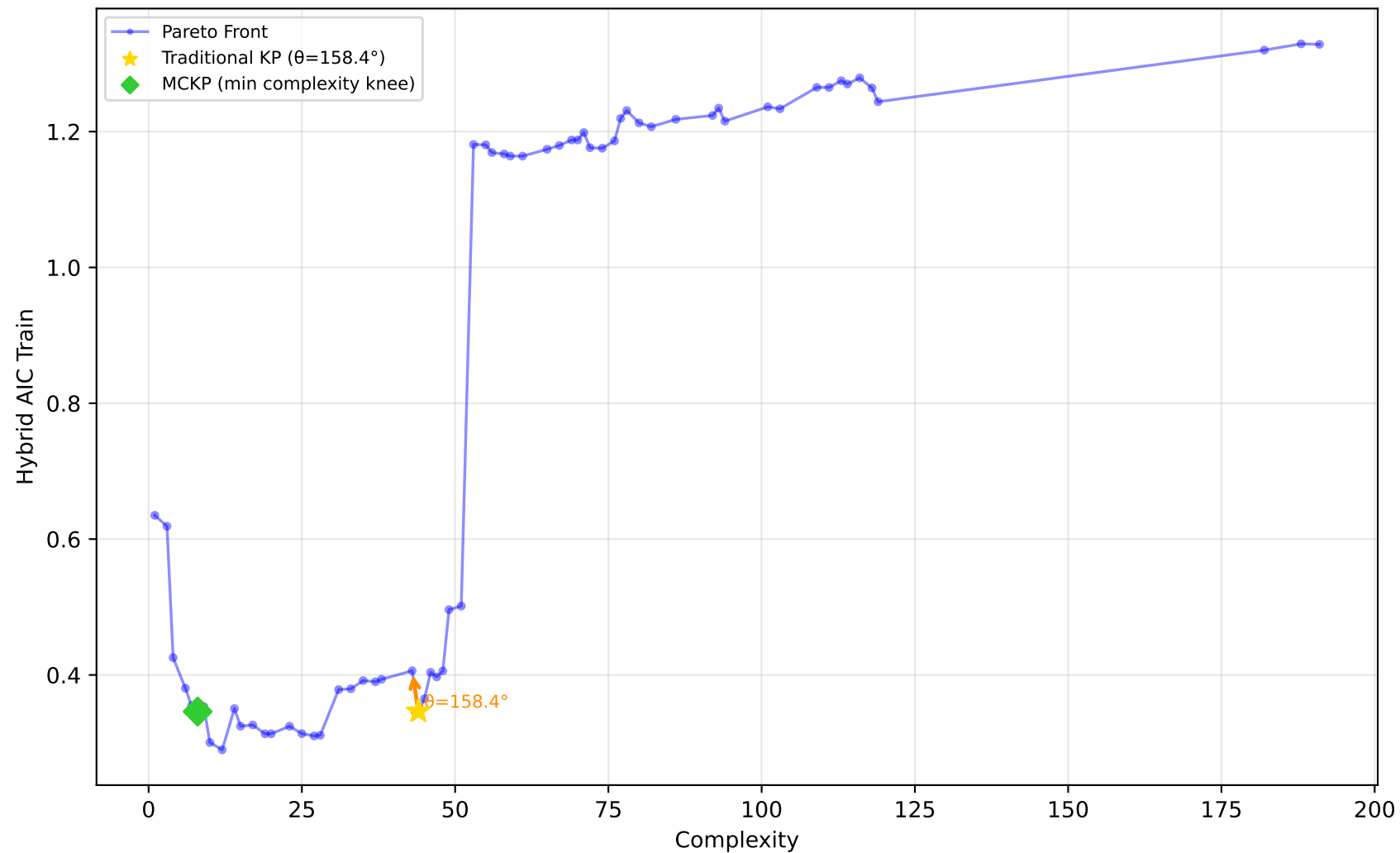
228_elusage - Run 6 - MVP - Hybrid AIC Train \lambda_1=0.00 , \lambda_2=0.00 , \lambda_3=1.00 | Difficulty: 0.41 | Method: mckp
