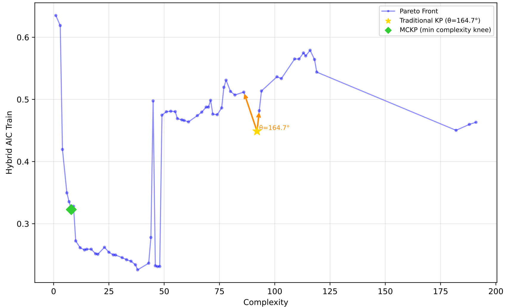
228_elusage - Run 6 - MVP - Hybrid AIC Train \lambda_1=0.00, \lambda_2=0.30, \lambda_3=0.00 | Difficulty: 0.41 | Method: mckp
