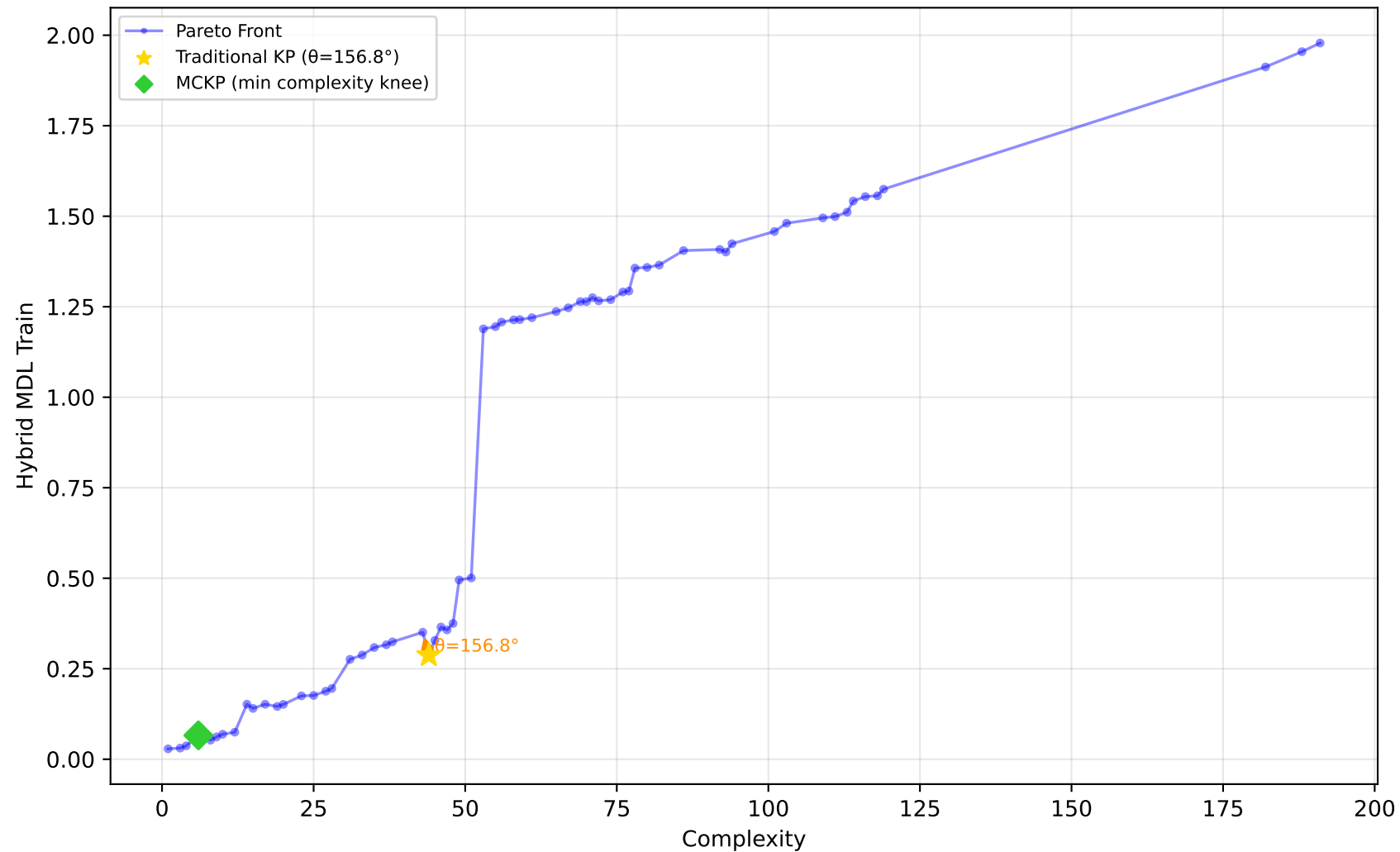
228_elusage - Run 6 - MVP - Hybrid MDL Train \lambda_1=0.00, \lambda_2=0.00, \lambda_3=1.00 | Difficulty: 0.41 | Method: mckp
