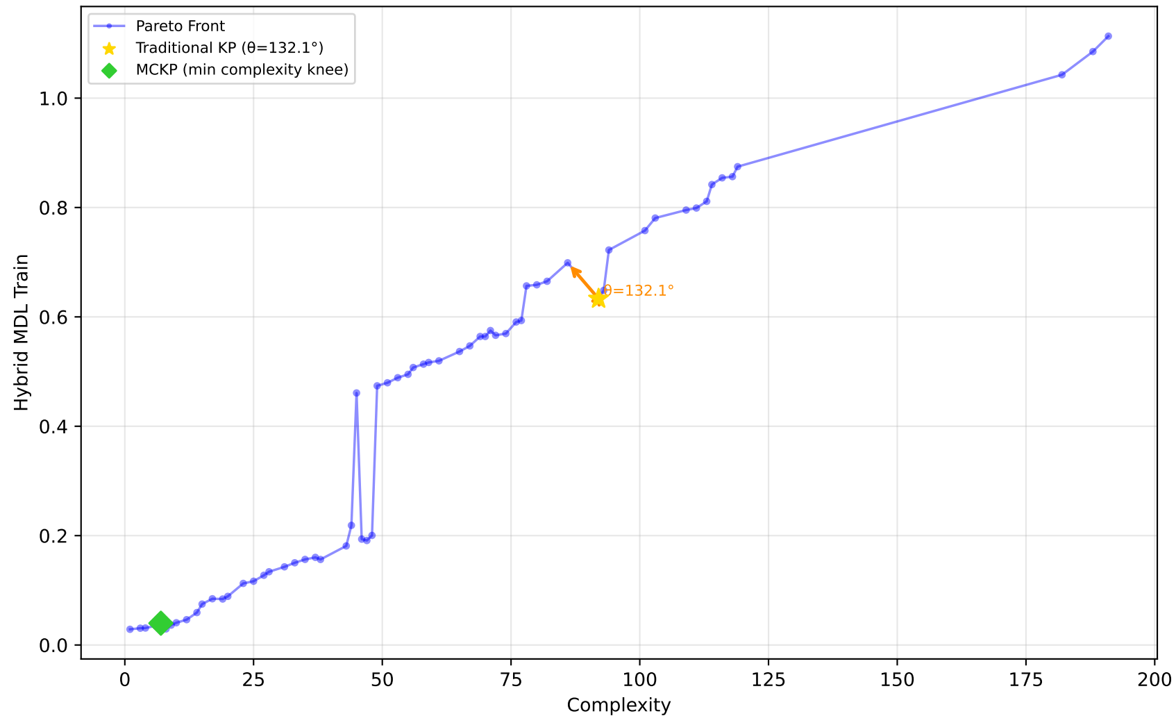
228_elusage - Run 6 - MVP - Hybrid MDL Train \lambda_1=0.00, \lambda_2=0.30, \lambda_3=0.00 | Difficulty: 0.41 | Method: mckp
