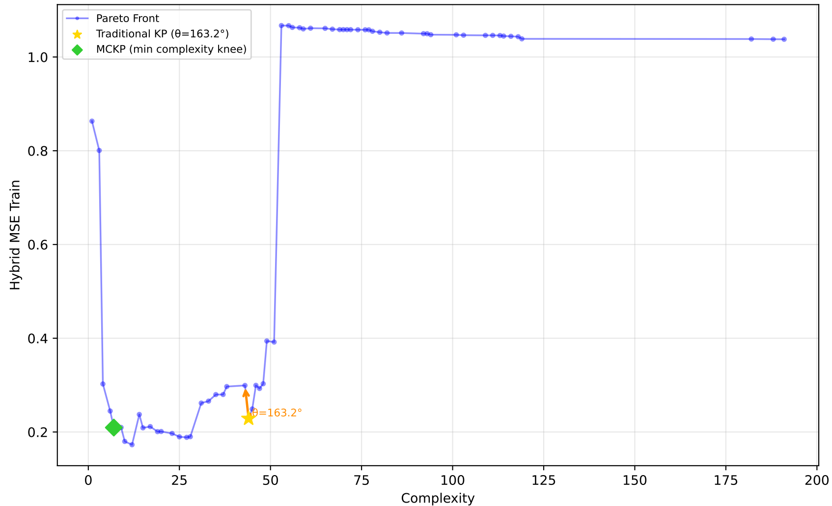
228_elusage - Run 6 - MVP - Hybrid MSE Train \lambda_1=0.00, \lambda_2=0.00, \lambda_3=1.00 | Difficulty: 0.41 | Method: mckp
