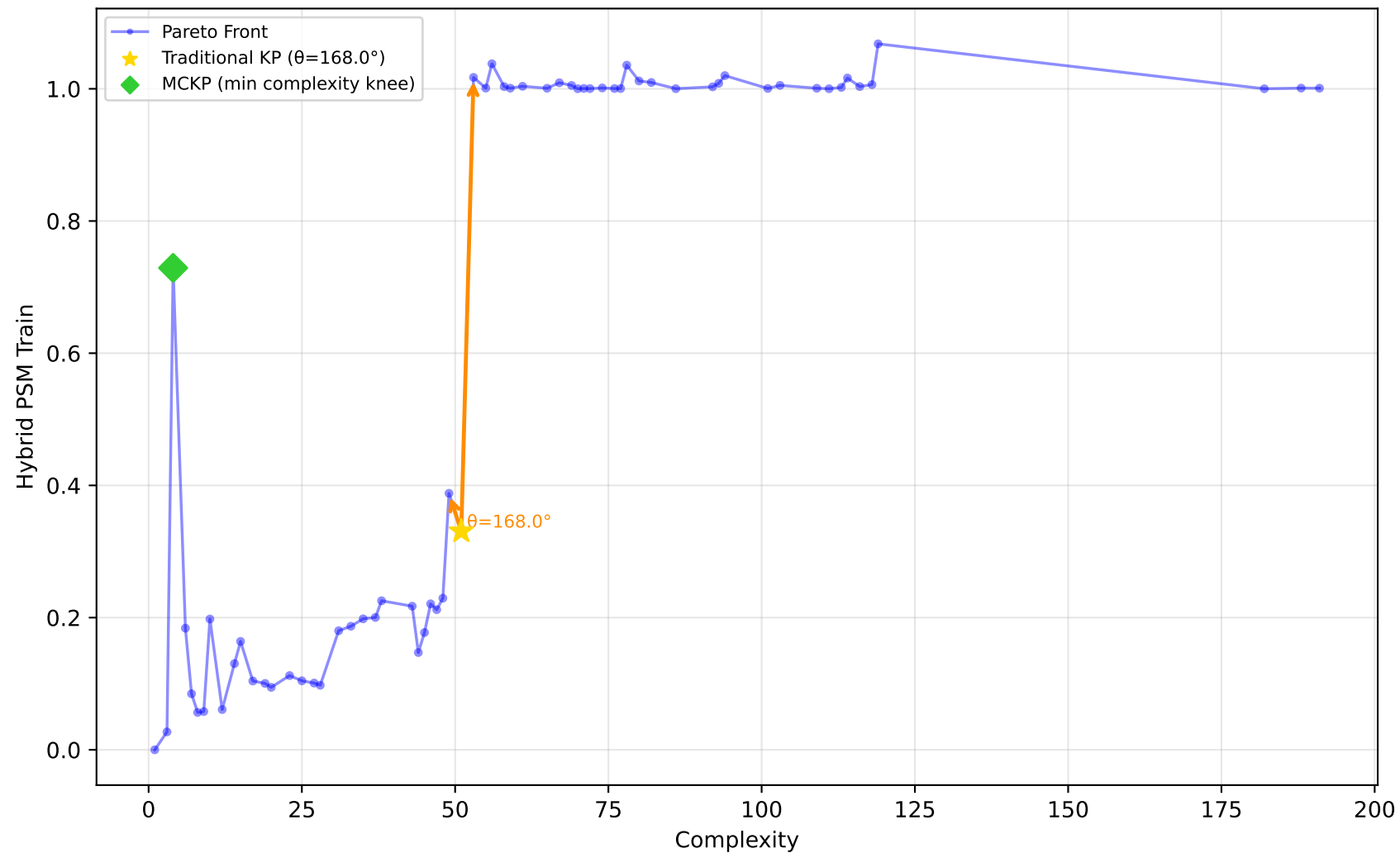
228_elusage - Run 6 - MVP - Hybrid PSM Train \lambda_1=0.00, \lambda_2=0.00, \lambda_3=1.00 | Difficulty: 0.41 | Method: mckp
