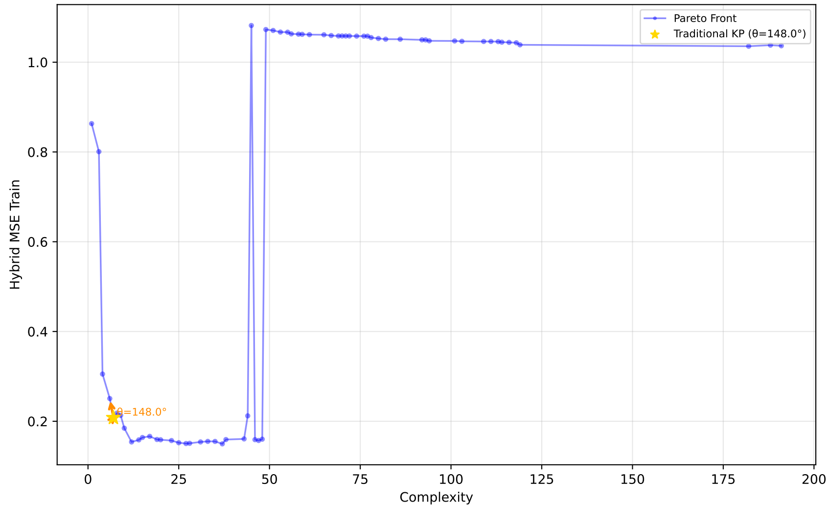
228_elusage - Run 6 - SVP - Hybrid MSE Train \lambda_1=0.00, \lambda_2=1.00, \lambda_3=0.00 | Difficulty: 0.41 | Method: mckp
