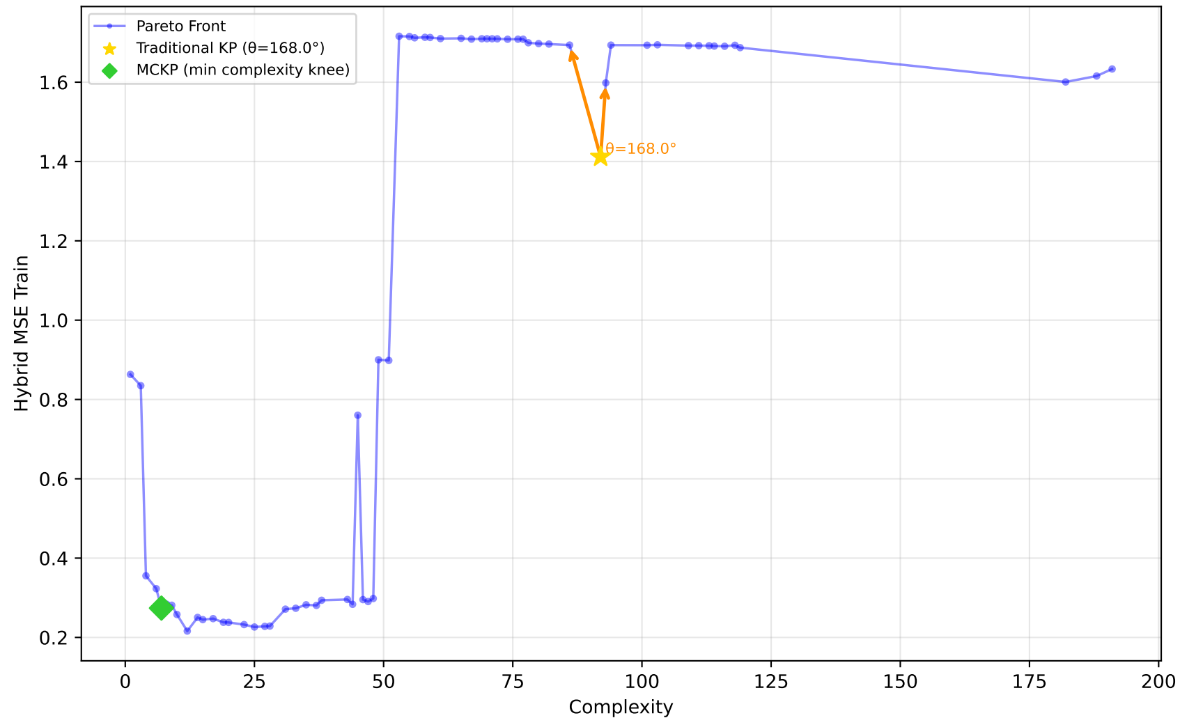
228_elusage - Run 6 - SVP - Hybrid MSE Train \lambda_1=0.60, \lambda_2=0.60, \lambda_3=1.00 | Difficulty: 0.41 | Method: mckp
