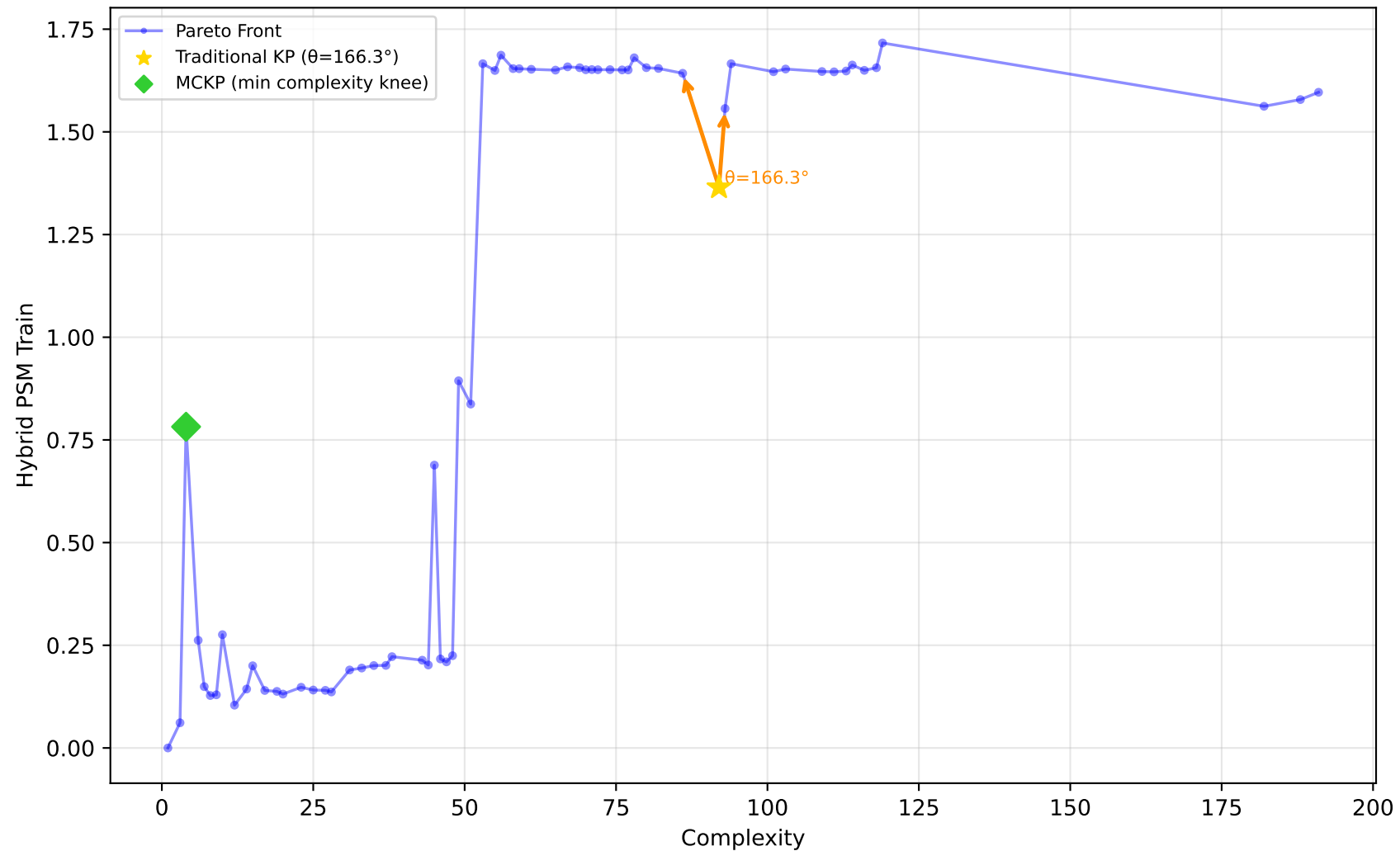
228_elusage - Run 6 - SVP - Hybrid PSM Train \lambda_1=0.60, \lambda_2=0.60, \lambda_3=1.00 | Difficulty: 0.41 | Method: mckp
